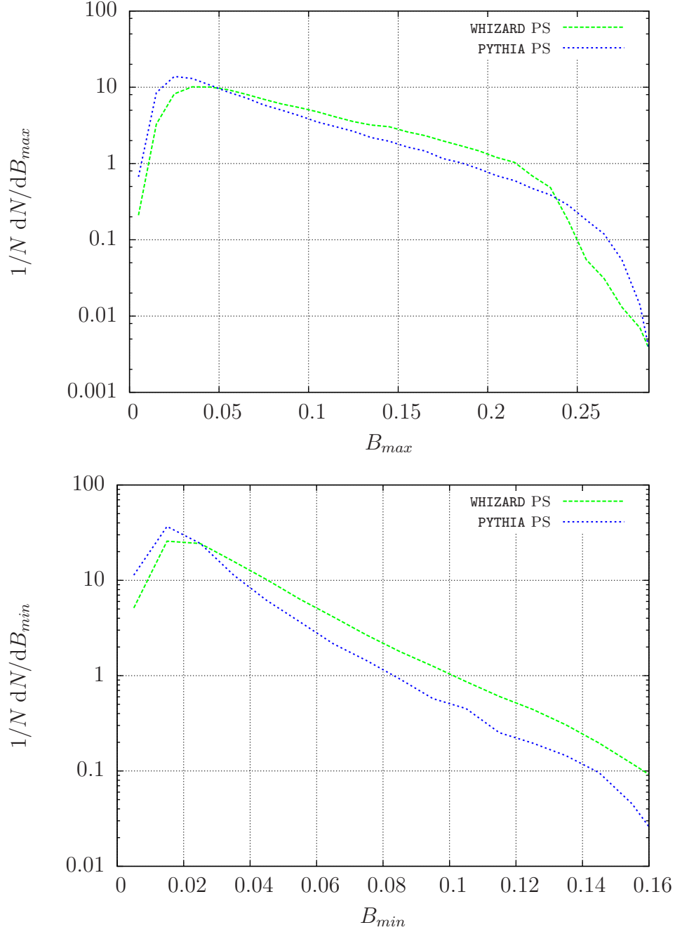
Figure 5.3: Plots for jet broadenings B_{max} and B_{min} (without hadronization). The dashed/green/bright line is WHIZARD, the dotted/blue/dark line is PYTHIA.
