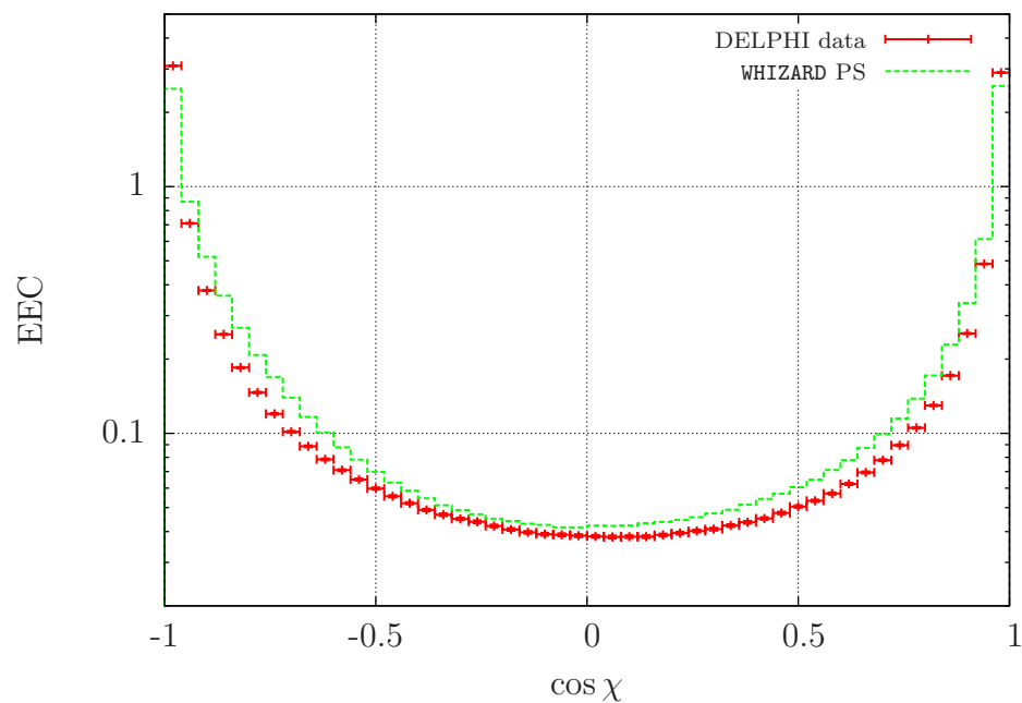
Figure 5.9: Plot for energy-energy correlation at LEP (with hadronization, data from [86], EEC calculated using Rivet [88]). The dashed/green/bright line is WHIZARD.
