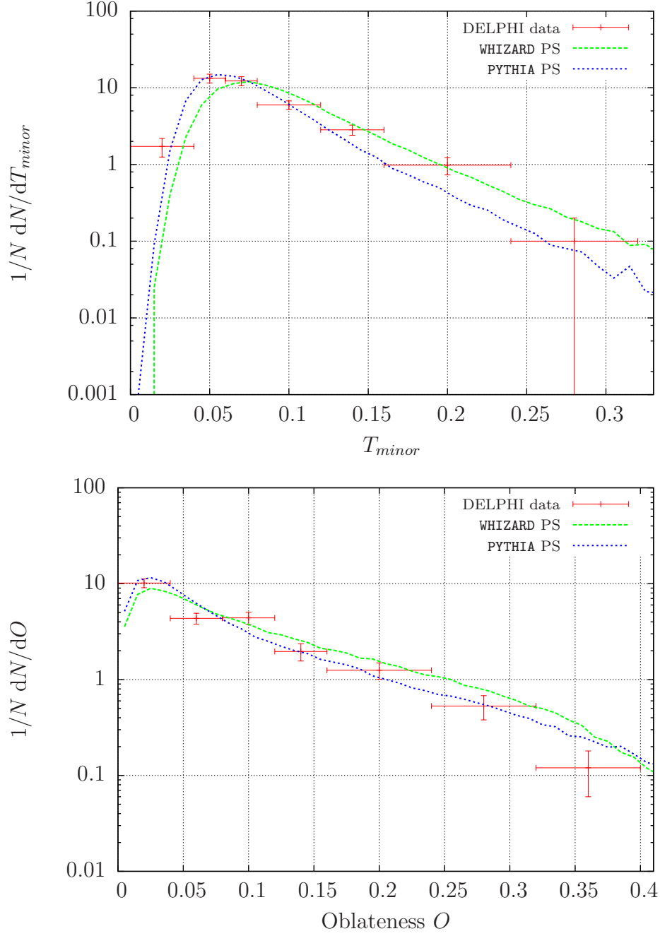
Figure 5.6: Plots for thrust minor T_{\text{minor}} and Oblateness O (with hadronization, data from [87]). The dashed/green/bright line is WHIZARD, the dotted/blue/dark line is PYTHIA.
