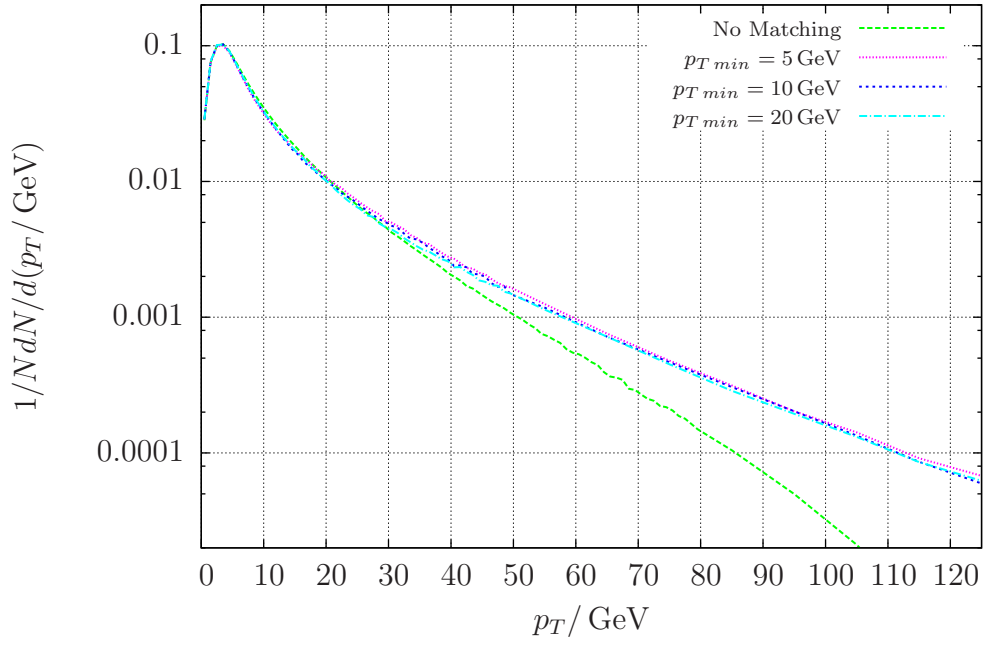
Figure 5.20: The “NoMatching” curve and the “Matching (1jet)” (cf. figure 5.19) curve for three different values of p_{T\min} (5 GeV, 10 GeV and 20 GeV).
