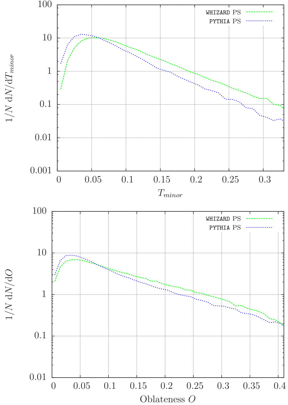
Figure 5.2: Plots for thrust minor T_{\text{minor}} and Oblateness O (without hadronization). The dashed/green/bright line is WHIZARD, the dotted/blue/dark line is PYTHIA.
