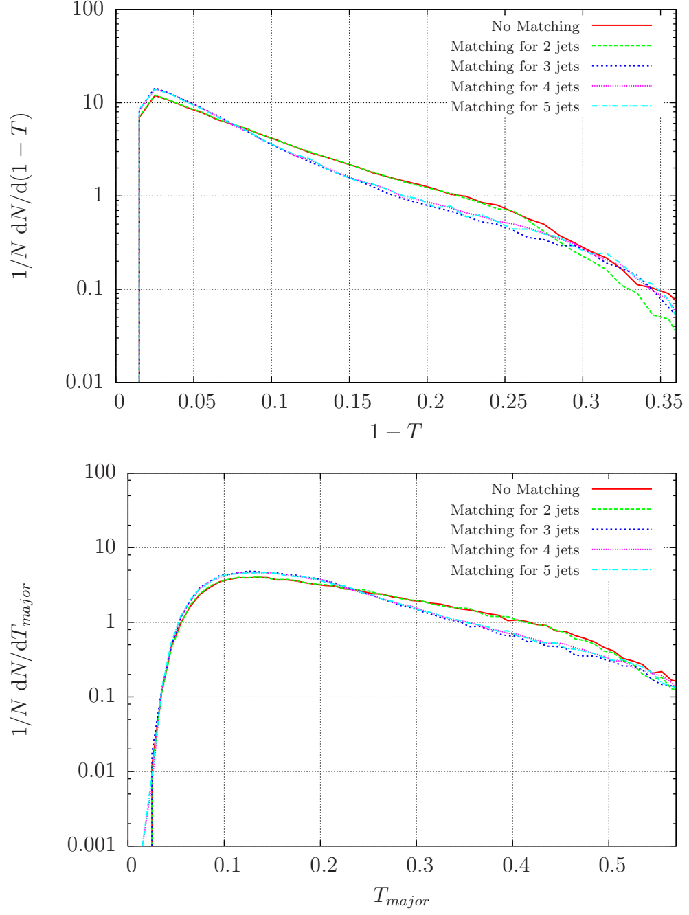
Figure 5.13: Plots for thrust T and thrust major T_{\text{major}} (WHIZARD ME + WHIZARD PS with matching).
