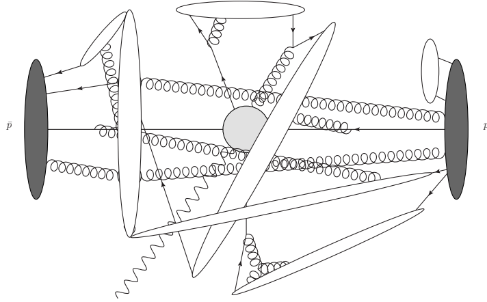
Figure 1.9: Generating an event: adding hadronization. The hadrons are shown as white ovals.
