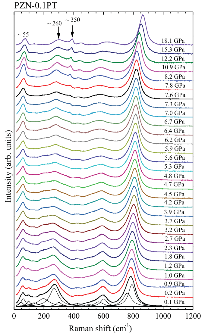
FIG. 5. (Color online) Raman spectra of PZN-0.1PT measured up to 18.1 GPa.
