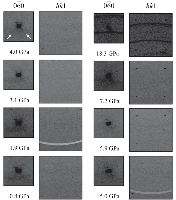
FIG. 3. Reciprocal-space layers reconstructed from synchrotron single-crystal XRD on PZN-0.1PT. The Miller indices refer to a cubic double-perovskite Fm\bar{3}m unit cell. The arrows in the sector around the 0\bar{6}0 Bragg peak mark the diffuse scattering along \langle 110 \rangle^* . The sectors of (hk1) layers demonstrate that pressure-induced odd-odd-odd Bragg peaks appear at 5.9 GPa; the reflections in the upper-right and bottom-right corner are \bar{1}\bar{3}1 and 1\bar{5}1 , respectively.
