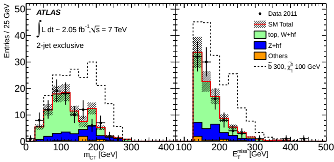
FIG. 1: Measured m_{CT} (left) and E_T^{\text{miss}} (right) distributions before the m_{CT} selection compared to the SM predictions (solid line) and SM+MSSM predictions (dashed lines). The dashed grey band represents the total systematic uncertainties.
