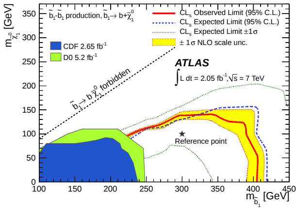
FIG. 2: Expected and observed exclusion limits, as well as \pm 1\sigma variation on the expected limit, in the \tilde{b}_1 - \tilde{\chi}_1^0 mass plane. The band around the observed limit delimited by the two dashed lines shows the effect of renormalization and factorization scale variation. The reference point indicated on the plane corresponds to the MSSM scenario with sbottom and neutralino masses of 300 GeV and 100 GeV, respectively. Results are compared to previous exclusion limits from Tevatron experiments. Results from LEP cover the region with sbottom mass below 100 GeV.
