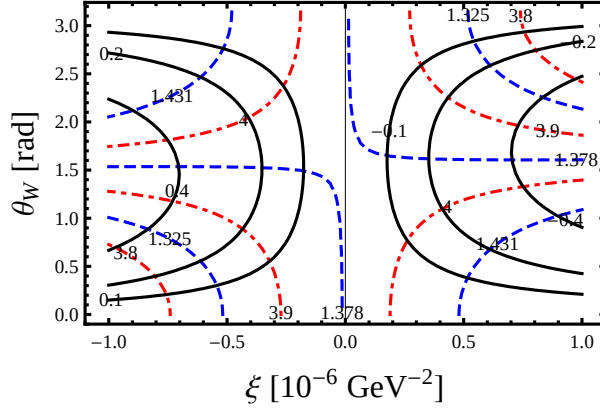
FIG. 3. Legend is the same as that in Fig. 2, but the magnitude of \Delta A_C^{dir} is smaller than the LHCb results of 1\sigma .
