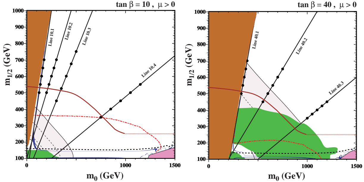
Fig. 2: The CMSSM (m_0, m_{1/2}) planes for (left) \tan \beta = 10, \mu > 0 and A_0 = 0 , and (right) \tan \beta = 40, \mu > 0 and A_0 = -500 GeV. In the brown shaded regions at small m_0 the LSP is charged, in the pink shaded regions at large m_0 there is no consistent electroweak vacuum, the green shaded regions are excluded by b \rightarrow s\gamma , and the grey shaded regions are favoured by (g - 2)_\mu at the 1- (2-) \sigma level indicated by dashed (solid) lines. LEP searches for charginos exclude the regions below the near-horizontal black dashed lines, LEP searches for the Higgs boson exclude the regions below the near-horizontal red dot-dashed lines, and LHC searches exclude the regions below the purple lines. The benchmark lines are solid black, and the dots denote the benchmark points spaced regularly along these lines. The dark blue strips yield the correct cold dark matter density in the CMSSM. All experimental numbers and the corresponding references can be found in [68].
