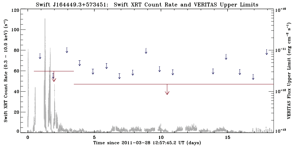
Figure 1. Flaring, low-state and daily upper limits are shown superimposed on the Swift XRT light curve (Evans et al. 2007). The extent of the daily upper limit horizontal bars represents the approximate time interval during which the VERITAS observations were taken.
