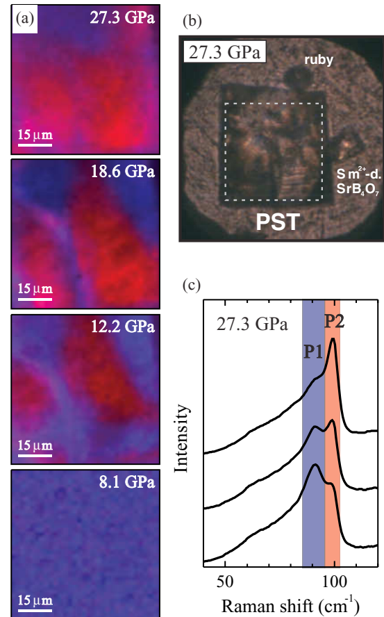
FIG. 4. (Color) Raman mappings (a) of single-crystal PST at different pressures based on the integrated intensity ratio between the signals P2 and P1 (c); red corresponds to large ratio I(P2)/I(P1) , blue to small ratio. The mapping area is marked by the white dashed square in the crystal image (b).
