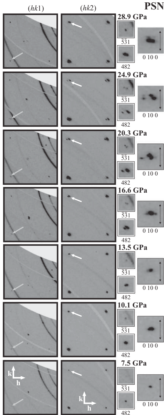
FIG. 6. Reciprocal-space layer sections of PSN reconstructed in Fm\bar{3}m from single-crystal synchrotron XRD data at different pressures. The reflection in the lower-left and upper-right corners are \bar{5}11 and \bar{3}31 for the (hk1) layer and 482 and 662 for the (hk2) layer, respectively. The gray and white arrows mark examples of the pressure-induced odd-odd-odd and even-even-even reflections, which are shown on an enlarged scale. The 0 10 0 reflection is also shown; the black vertical arrows in the 0 10 0-layer sections mark the direction to the coordinate origin.
