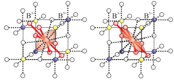
FIG. 1. (Color online) A sketch of \text{PbB}_{0.5}^{3+}\text{B}_{0.5}^{5+}\text{O}_3 compound with local chemical 1:1 B-site order (left-hand side) and disorder (right-hand side). The reddish ellipses represent the anisotropic displacement ellipsoids of \text{Pb}^{2+} cations.
