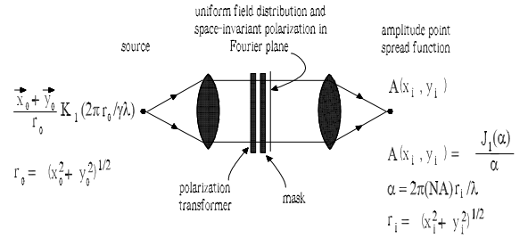
Figure 10: OTR particle spread function synthesis by a Fourier-plane filter and a polarization transformer.
