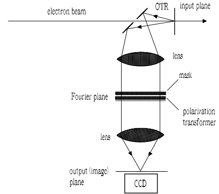
Figure 5: A practical arrangement of the coherent OTR image-processing system.
