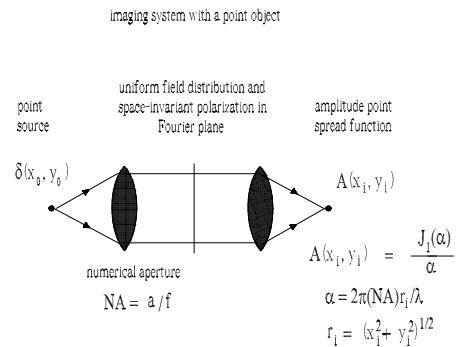
Figure 7: Two-lens imaging system with a point source.
