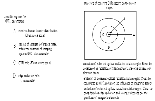
Figure 3: Scheme of the coherent OTR radiation pattern as observed in the object plane for the low electron beam energy case of 2 GeV.
