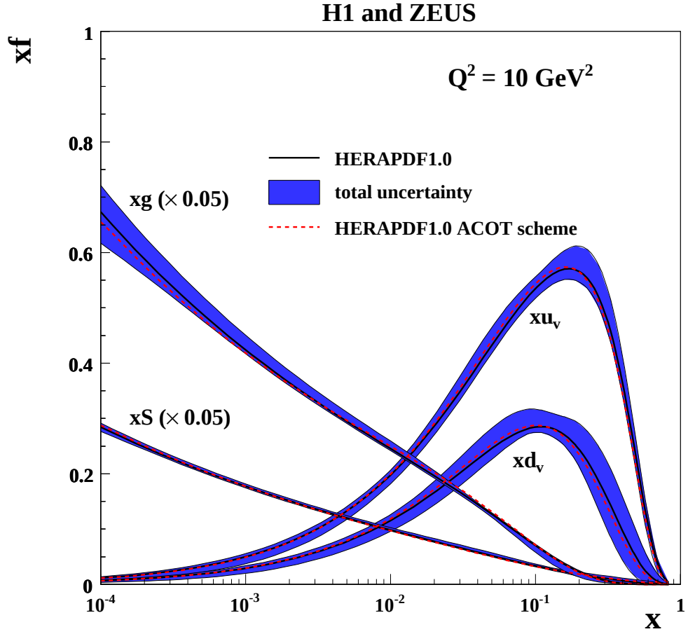
Figure 20: The parton distribution functions obtained using ACOT heavy-flavour scheme compared to HERAPDF1.0 for xu_v , xd_v , xS = 2x(\bar{U} + \bar{D}) , xg , at Q^2 = 10 \text{ GeV}^2 . The bands show total uncertainties of the HERAPDF1.0 fit.
