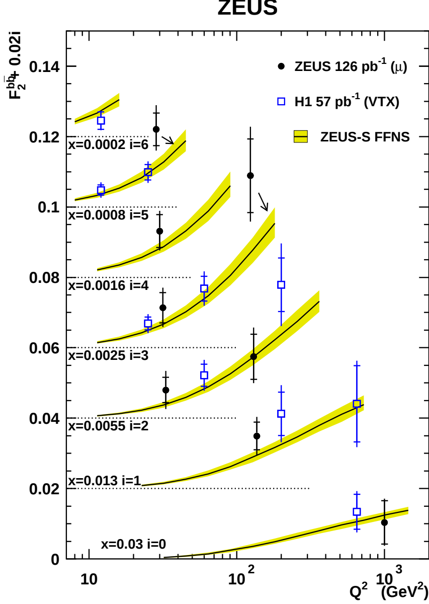
Figure 7: The structure function F_2^{bb} (filled symbols) plotted as a function of Q^2 for fixed x values. The curves represent the NLO QCD predictions in the FFNS using the ZEUS-S PDF fit. The inner error bars are the statistical uncertainty while the outer bars represent the statistical, systematic and theoretical uncertainties added in quadrature. The band represents the uncertainty on the NLO QCD prediction. All the previous data (open symbols) are also shown, corrected to the reference x values used in this analysis: 0.0005 \rightarrow 0.0008 , 0.002 \rightarrow 0.0025 , 0.005 \rightarrow 0.0055 , 0.032 \rightarrow 0.030 .
