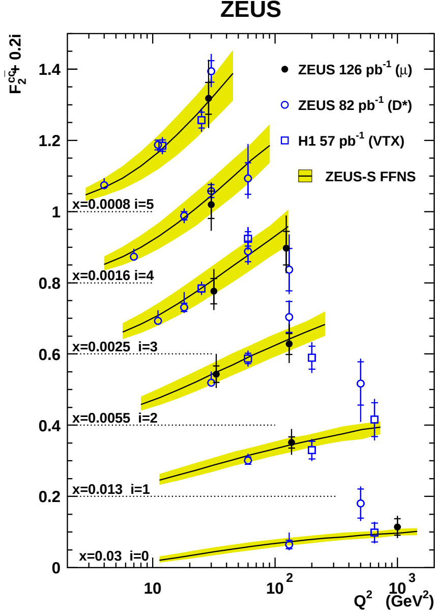
Figure 6: The structure function F_2^{c\bar{c}} (filled symbols) plotted as a function of Q^2 for fixed x values. The curves represent the NLO QCD predictions in the FFNS using the ZEUS-S PDF fit. The inner error bars are the statistical uncertainty while the outer bars represent the statistical, systematic and theoretical uncertainties added in quadrature. The band represents the uncertainty on the NLO QCD prediction. A selection of previous data (open symbols) is also shown, corrected to the reference x values used in this analysis: ZEUS D^* : 0.001 \rightarrow 0.0008, 0.0015 \rightarrow 0.0016, 0.003 \rightarrow 0.0025, 0.006 \rightarrow 0.0055, 0.012 \rightarrow 0.013; H1 VTX: 0.0005 \rightarrow 0.0008, 0.002 \rightarrow 0.0025, 0.005 \rightarrow 0.0055, 0.032 \rightarrow 0.030.
