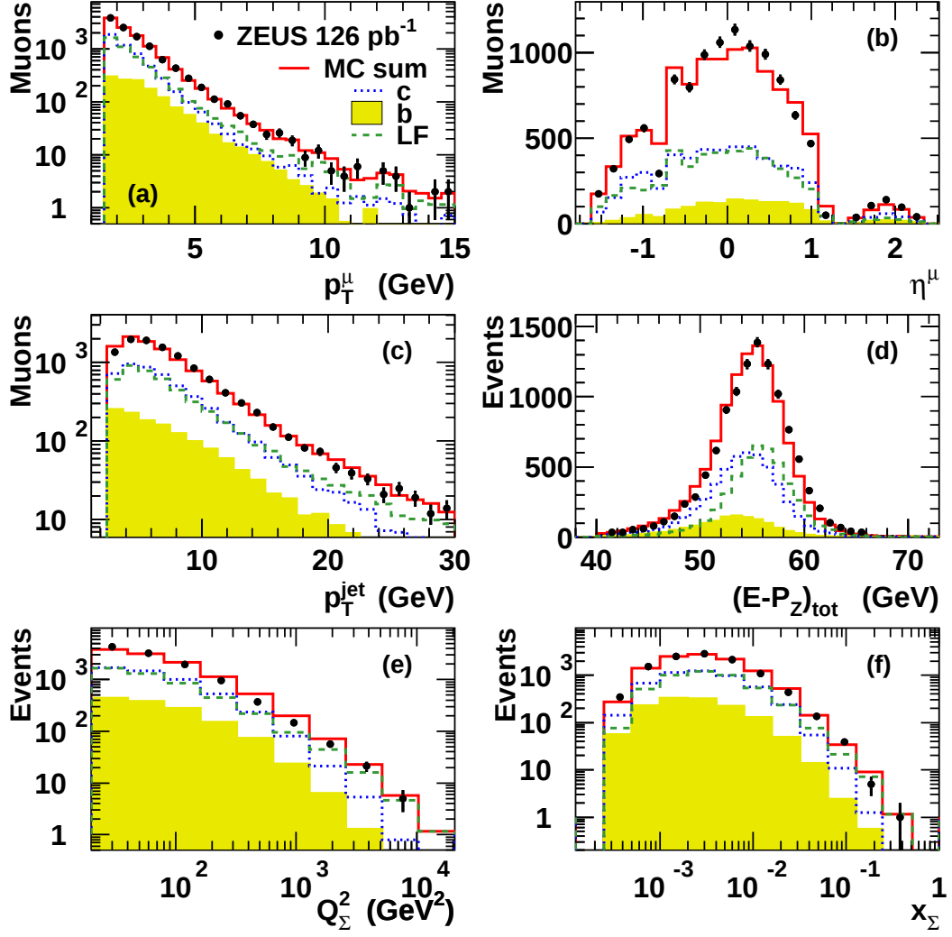
Figure 2: Distributions of (a) p_T^\mu , (b) \eta^\mu , (c) p_T^{\text{jet}} , (d) (E-P_Z)_{\text{tot}} , (e) Q_\Sigma^2 and (f) x_\Sigma for the selected sample of muons in DIS. The data (points) are compared to the MC expectation with the normalisation of the c, b and light flavours, LF, components obtained from the global fit.
