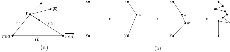
Fig. 4. (a) The transverse colour-electric field in a colour dipole. (b) Gluon emission splits the dipole into two dipoles. Repeated emissions give a cascade, which produces a chain of dipoles.
