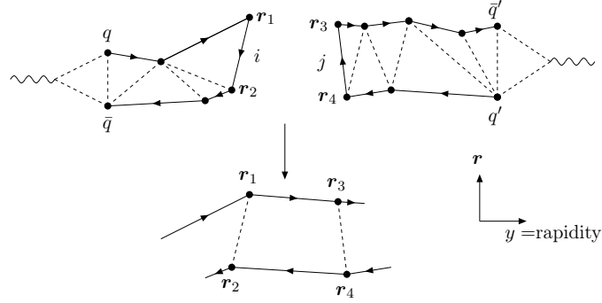
Fig. 5. A symbolic picture of a \gamma^*\gamma^* collision in y - r_\perp -space. When two colliding dipoles interact via gluon exchange the colors are reconnected forming dipole chains stretched between the remnants of the colliding systems.
