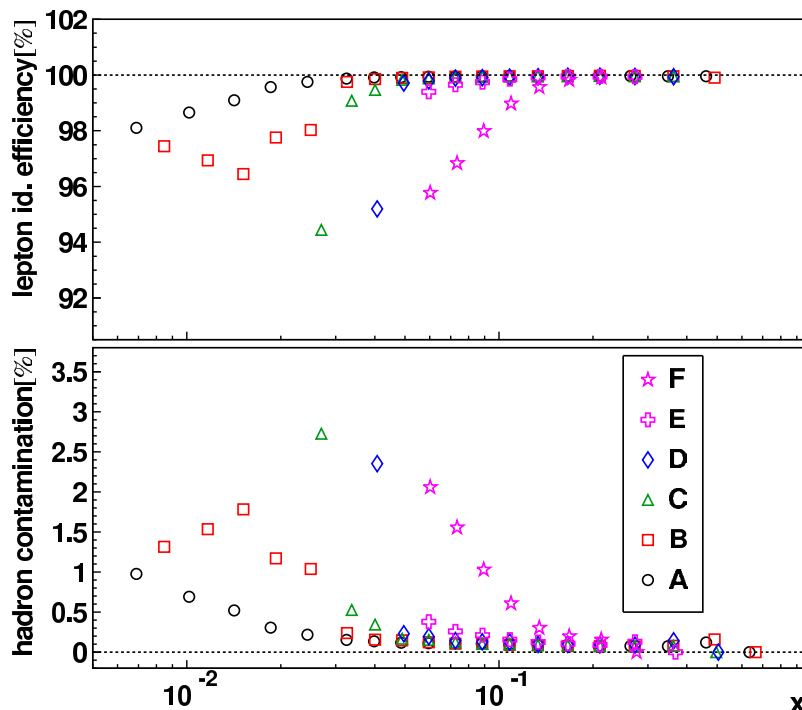
Figure 3. Lepton identification efficiency \mathcal{E}_{\text{lep}} and hadron contamination \mathcal{C}_{\text{had}} in the year 2000. The symbols refer to the Q^2 binning shown in figure 1.
