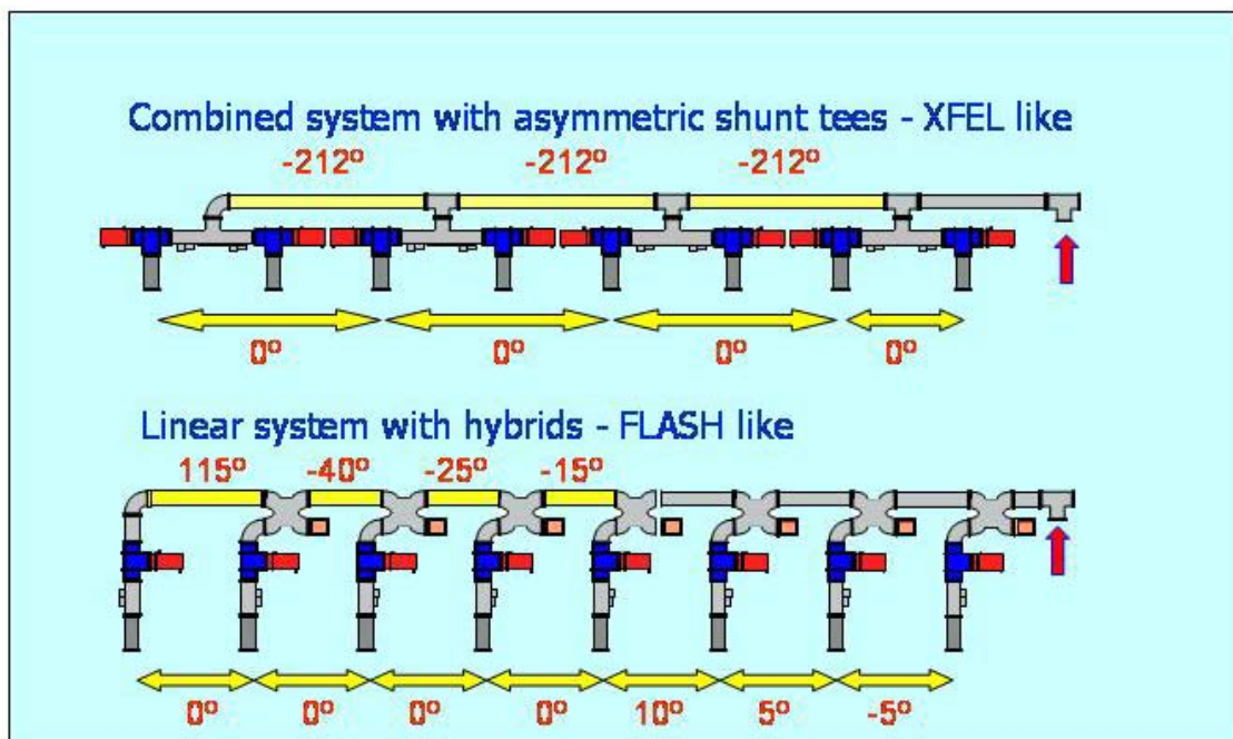
Fig. 4: Combined and linear RF waveguide distribution system
