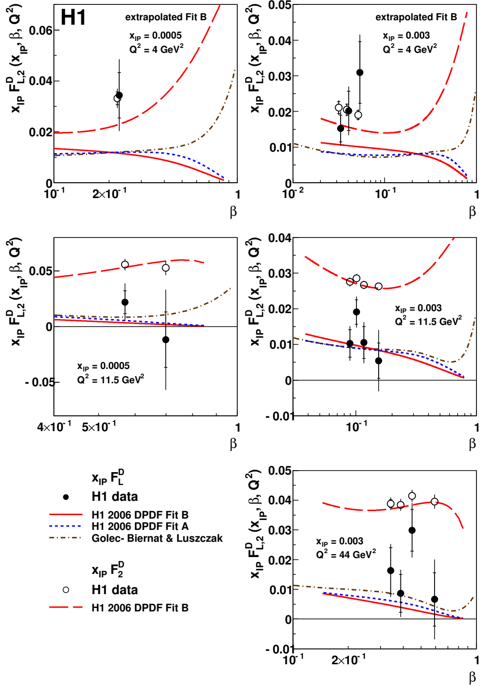
Figure 7: The diffractive structure functions F_L^D and F_2^D multiplied by x_{\text{IP}} as a function of \beta at fixed Q^2 and x_{\text{IP}} . The F_L^D data are shown as filled points, compared with the predictions of H1 2006 DPDF Fit A (dashed line), Fit B (solid line) and the Golec-Biernat and Łuszczak model (dashed and dotted line). The measurements of F_2^D (open points) are compared with the prediction of H1 2006 DPDF Fit B (long dashed line). The inner error bars represent the statistical uncertainties on the measurement, the outer error bars represent the statistical and total systematic uncertainties added in quadrature. The normalisation uncertainty of 8.1% is not shown.
