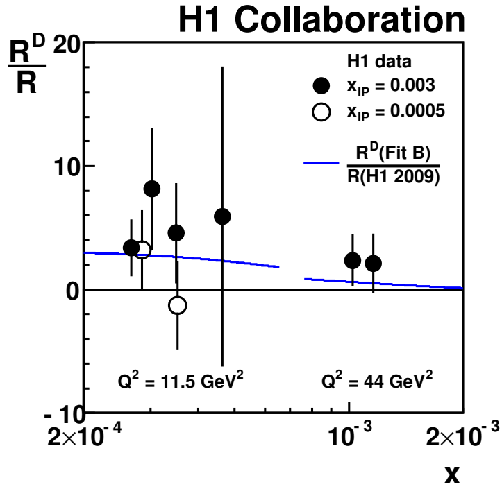
Figure 10: The ratio of R^D/R as a function of x at the indicated values of Q^2 and x_{IP} . The data are compared with the predicted ratio using H1 2006 DPDF Fit B / H1 PDF 2009 (solid line). The error bars represent the statistical and systematic uncertainties added in quadrature.
