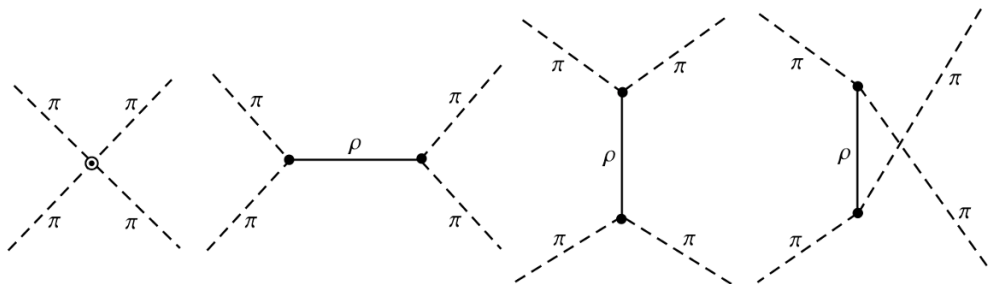
Figure 1. Feynman diagrams contributing to the \pi\pi \rightarrow \pi\pi scattering.
