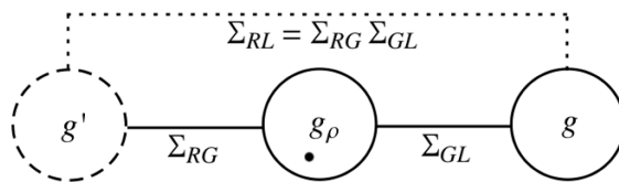
Figure 10. Moose diagram for the most general three-site model.
