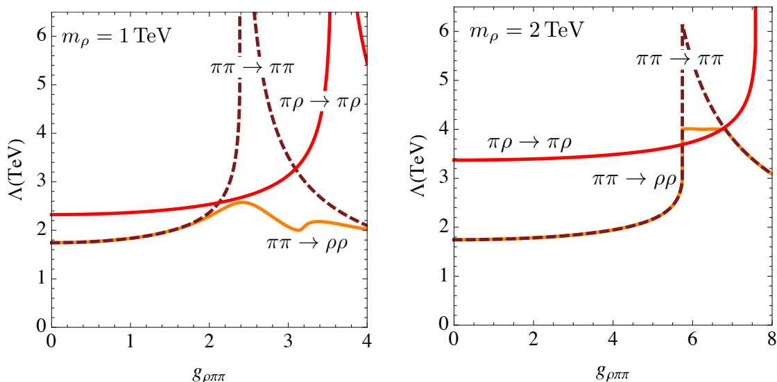
Figure 4. The maximal cutoff scale allowed by unitarity in the \pi\pi \rightarrow \pi\pi (dashed brown), \pi\pi \rightarrow \rho\rho (orange), and \pi\rho \rightarrow \pi\rho (red) channels for m_\rho = 1 TeV (left) and m_\rho = 2 TeV (right) as a function of the \rho\pi\pi coupling. The optimal for unitarity “turnaround” region in the \pi\pi \rightarrow \pi\pi amplitude (explained in the text) is clearly distinguishable. Note that in the limit g_{\rho\pi\pi} \rightarrow 0 , we recover the cutoff of the SM without the Higgs boson, 1.7 TeV.
