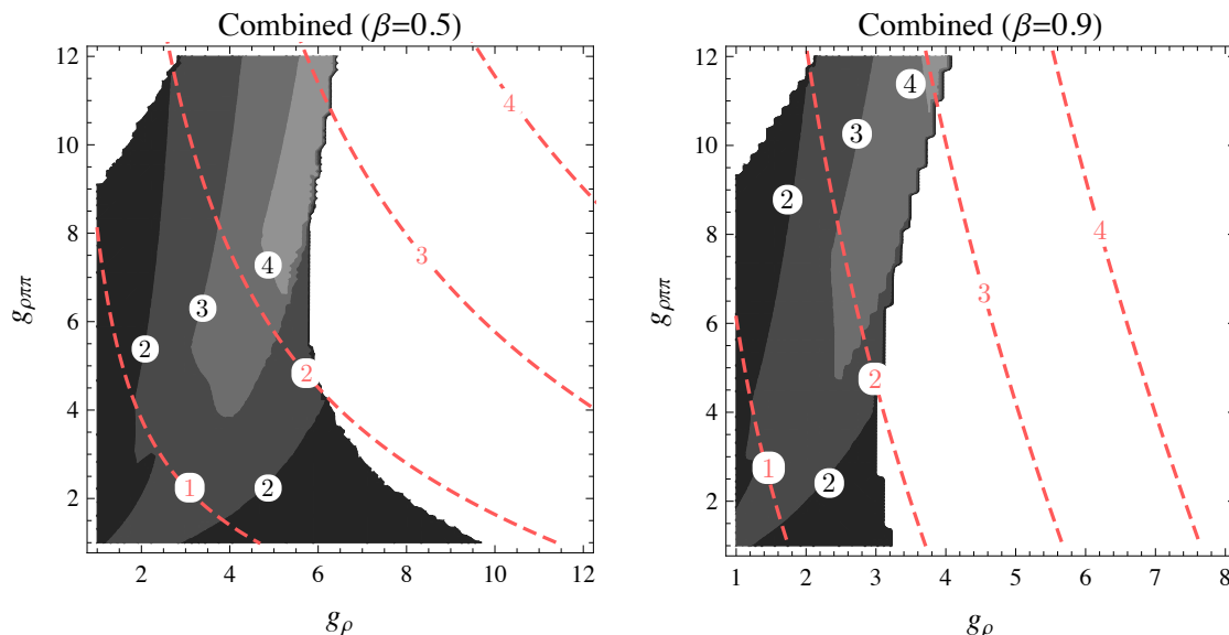
Figure 8. Contour plots of the maximum cut-off scale for \beta = 0.5 (left) and \beta = 0.9 (right) overlaid it with contours of constant m_\rho (dashed). The shaded regions correspond to a cutoff scale \Lambda smaller than 2, 3, 4 TeV (from dark to light gray).
