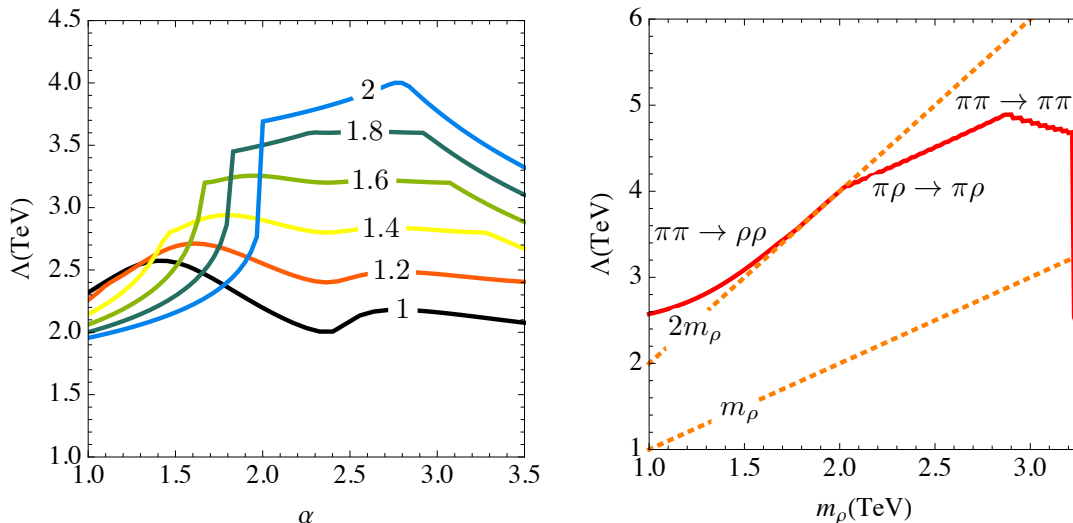
Figure 5. The maximal cutoff scale allowed by unitarity (summing all considered channels) for several values of m_\rho [TeV] as a function of \alpha (left) and the maximal possible value of the cutoff as a function of m_\rho (right). Again, at fixed m_\rho , in the limit \alpha \rightarrow 0 we recover the cutoff of the SM without the Higgs boson.
