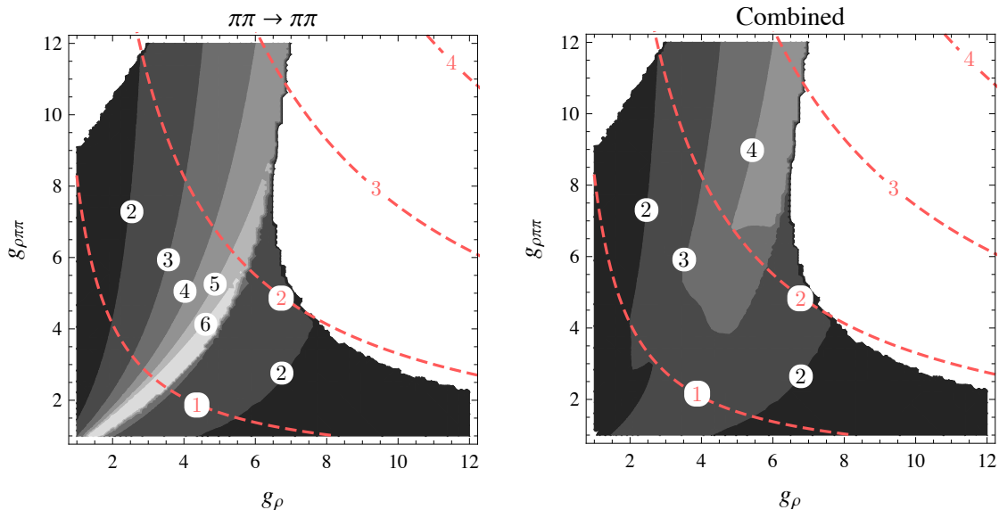
Figure 2. Contour plots for maximum cut-off scale allowed by the unitarity of the \pi\pi \rightarrow \pi\pi channel (left), and by all 2-to-2 channels combined (right), overlaid with contours of constant m_\rho/\text{TeV} (red dashed), The colored regions correspond to a cutoff scale \Lambda smaller than 2, 3, 4, 5, 6 TeV (from dark to light gray).
