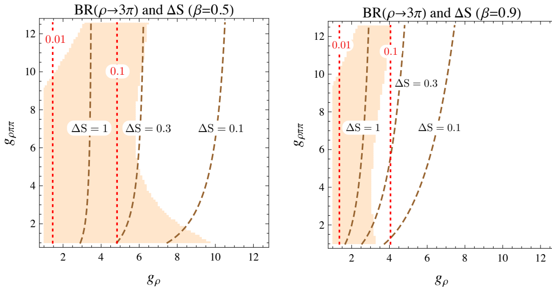
Figure 9. The parameter space allowed by the unitarity constraints (light orange) overlaid with contours of the constant \text{Br}(\rho \rightarrow 3\pi) (dotted) and \Delta S (dashed) for \beta = 0.5 (left) and \beta = 0.9 (right).
