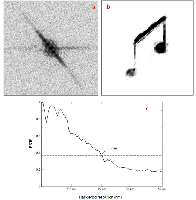
FIG. 3 (color online). Single-shot coherent soft x-ray diffraction patterns and the reconstructed image. (a) Measured diffracted intensity from the sample, in logarithmic scale, obtained in single-shot acquisition (20 fs exposure time). The maximal spatial frequency at the edge of the diffraction pattern is 8.4 \mu\text{m}^{-1} . (b) Image of reconstructed object amplitude obtained with 59 nm pixel size. Despite less quality, the single-shot object reconstruction shows a qualitative agreement with the multishot reconstruction. In particular, the amplitude transmission is lower on the round of the left harmonic note. (c) PRTF function of the reconstructed image. The 1/e criteria value provides a half-period resolution length image of 119 nm.
