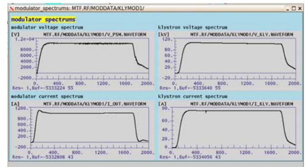
Figure 2: Voltage and current pulses at modulator output and klystron collector
