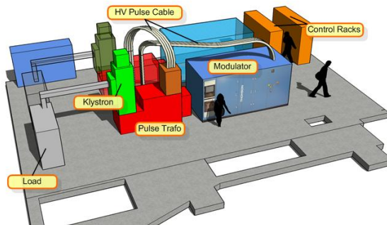
Figure 2: Layout of the MTF test setup
