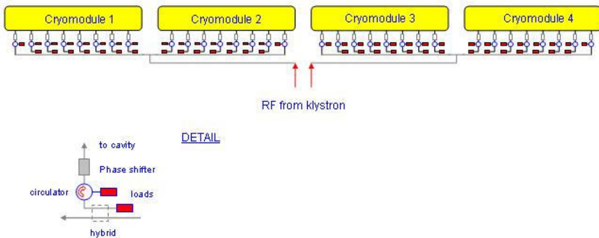
Fig. 1: Principle of an RF power transport system proposed for the TESLA linear collider
