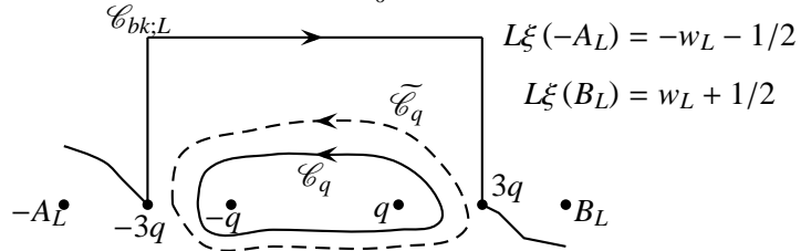
Figure 5: Contour \mathcal{C}_{bk:L} appearing in the definition of O^{(L)}[\nu, E_-^2](\lambda) , contour \mathcal{C}_q (solid line) and contour \tilde{\mathcal{C}}_q (dashed line). The contour \mathcal{C}_{bk:L} is such that, for |\Re \lambda| \geq 4q , it stays uniformly away from the real axis.
