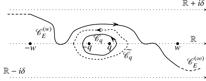
Figure 6: The contour \mathcal{C}_E^{(w)} consists of the solid line. The contour \mathcal{C}_E^{(\infty)} corresponds to the union of the solid and dotted lines. The loop \mathcal{C}_q is depicted in solid lines whereas the loop \tilde{\mathcal{C}}_q is depicted in dotted lines.
