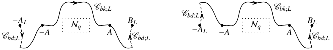
Figure 4: Contours \mathcal{C}_{bk;L} (solid lines) and \mathcal{C}_{bd;L} (dashed lines) in the case of k odd ( lhs ) and k even ( rhs ) in the case C_1 < 0 . The dotted lines \mathcal{C}_{bd;L} are pre-images of the segments [\epsilon_v w_L + \epsilon_v 1/2; \epsilon_v w_L + \epsilon_v 1/2 + i\epsilon' \alpha] , with v \in \{l, r\} and \epsilon_l = -1 and \epsilon_r = 1 . The sign of \epsilon' depends on the left or right boundary, the parity of k and the sign of C_1 .
