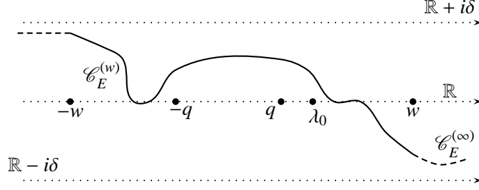
Figure 2: The contour \mathcal{C}_E^{(w)} consists of the solid line. The contour \mathcal{C}_E^{(\infty)} corresponds to the union of the solid and dotted lines. The localization of the saddle-point \lambda_0 corresponds to the space-like regime. Both contours lie in U_{\delta/2} .
