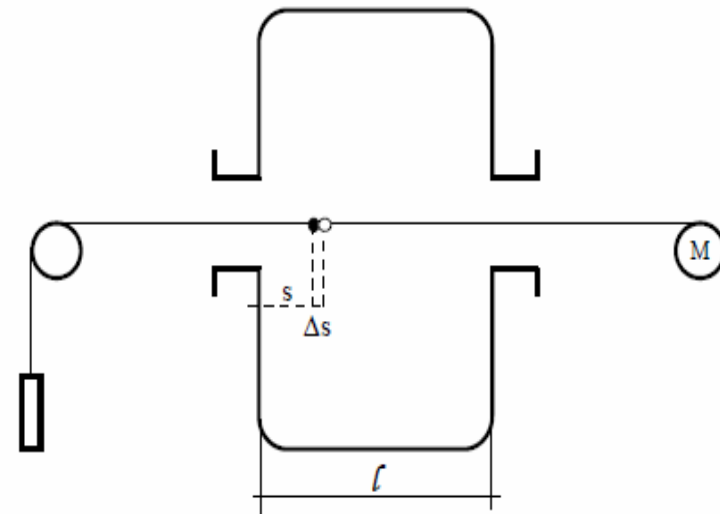
Schematic of a bead-puller apparatus
