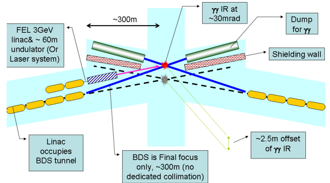
Figure 1: Conceptual configuration of Beam Delivery System, tunnels and location of FEL for the first 180GeV CM \gamma\gamma stage of a staged linear collider [7].
