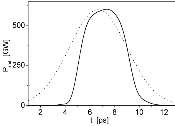
Figure 3: Temporal structure of the radiation pulse from FEL amplifier. Dashed line shows electron bunch profile. Radiation wavelength is 530 nm.
