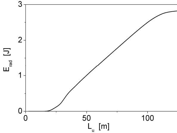
Figure 2: Energy in the FEL pulse versus undulator length.
