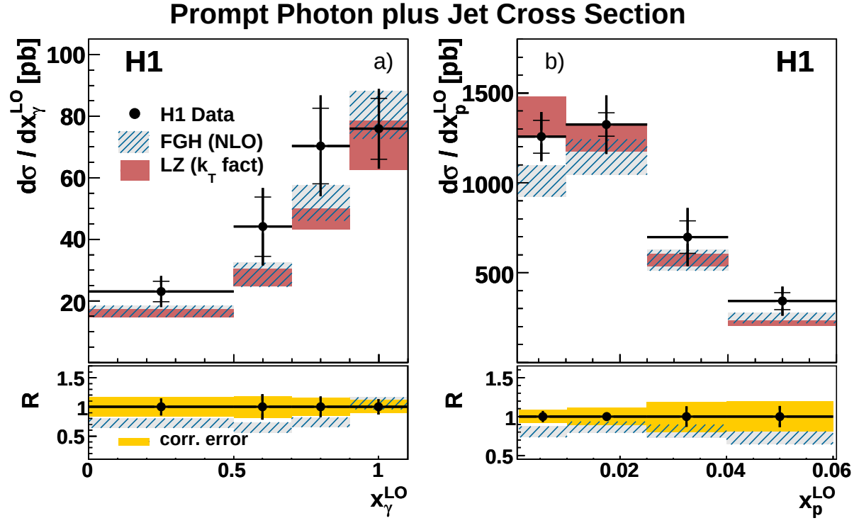
Figure 8: Differential prompt photon plus jet cross sections a) d\sigma/dx_{\gamma}^{LO} and b) d\sigma/dx_p^{LO} , in the kinematic range specified in table 1. The cross sections are compared to theoretical calculations (see caption figure 5).
