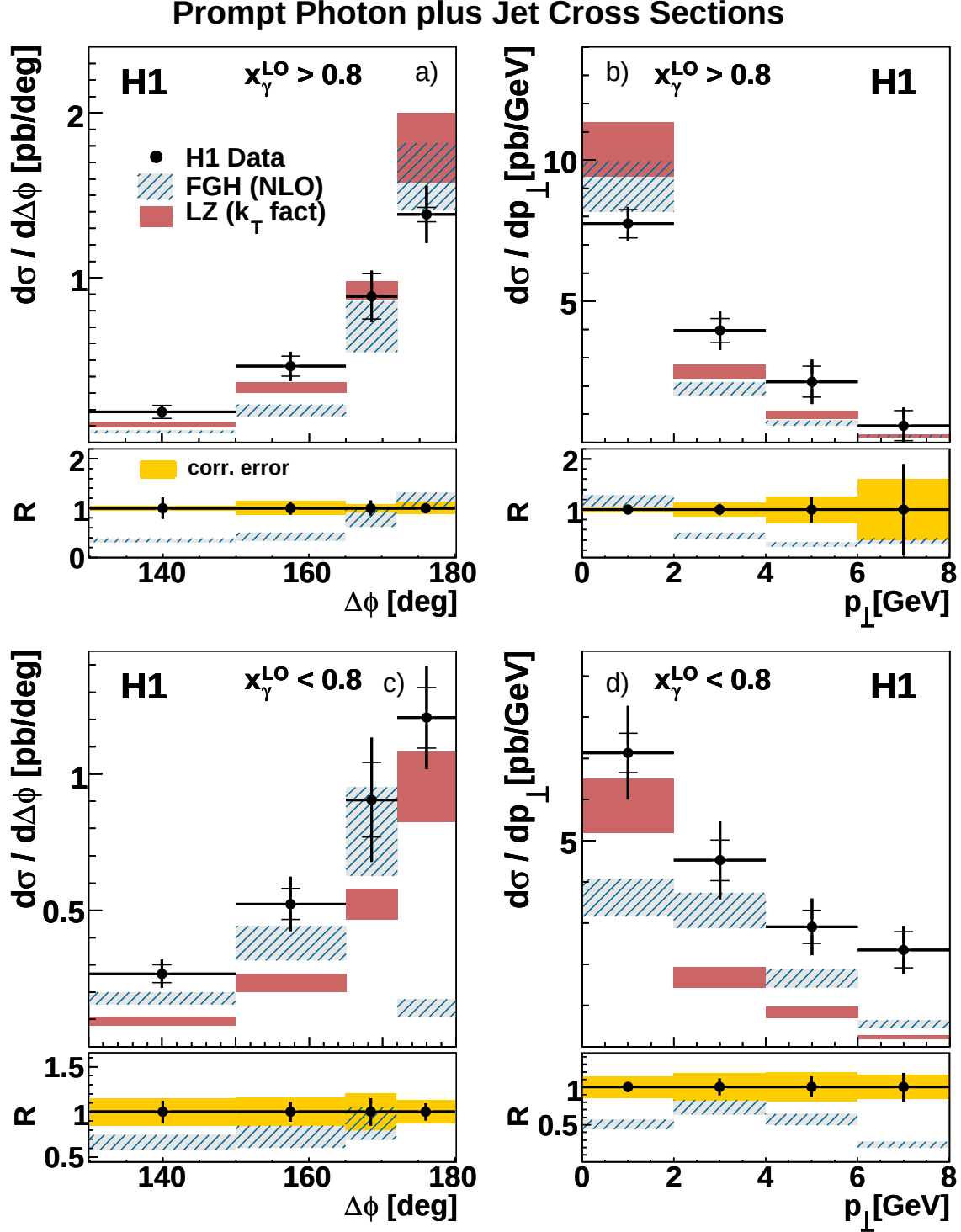
Figure 9: Differential prompt photon plus jet cross sections d\sigma/d\Delta\Phi and d\sigma/dp_\perp the photon momentum transverse to the jet direction, the difference in azimuthal angle between the photon and the jet. The kinematic range is specified in table 1. Figures a) and b) show the cross section for x_\gamma^{LO} > 0.8 , c) and d) for x_\gamma^{LO} < 0.8 . The cross sections are compared to theoretical calculations (see caption figure 5).
