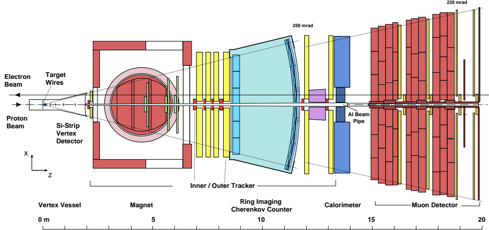
Figure 1: Top view of the HERA-B detector.
