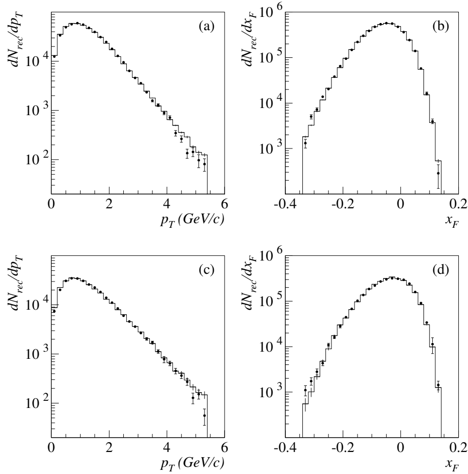
Figure 3: Distribution of the number of J/\psi s reconstructed in the carbon target sample (points) and in the corresponding MC data (histograms, arbitrarily re-normalized) as a function of p_T and x_F . (a) and (b): muon channel, (c) and (d): electron channel.
