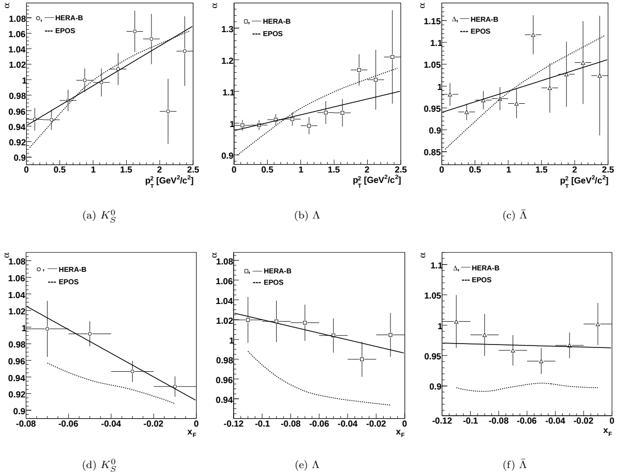
Figure 5: The dependence of \alpha for K_S^0 , \Lambda and \bar{\Lambda} production on p_T^2 (top plots) and x_F (bottom plots). The points show the measured values and the solid lines are the results of straight-line fits to the data. EPOS calculations are shown as dotted lines. The uncertainties include both statistical and systematic contributions.
