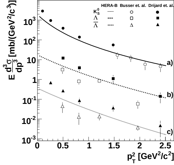
Figure 8: The average invariant cross section in the |y| \lesssim 1 interval for K_S^0 , \Lambda , and \bar{\Lambda} multiplied by the following scale factors: a) 600, b) 30, c) 1. The points are from [21] and [50]. The curves correspond to parameterizations of the present measurements as explained in the text.
