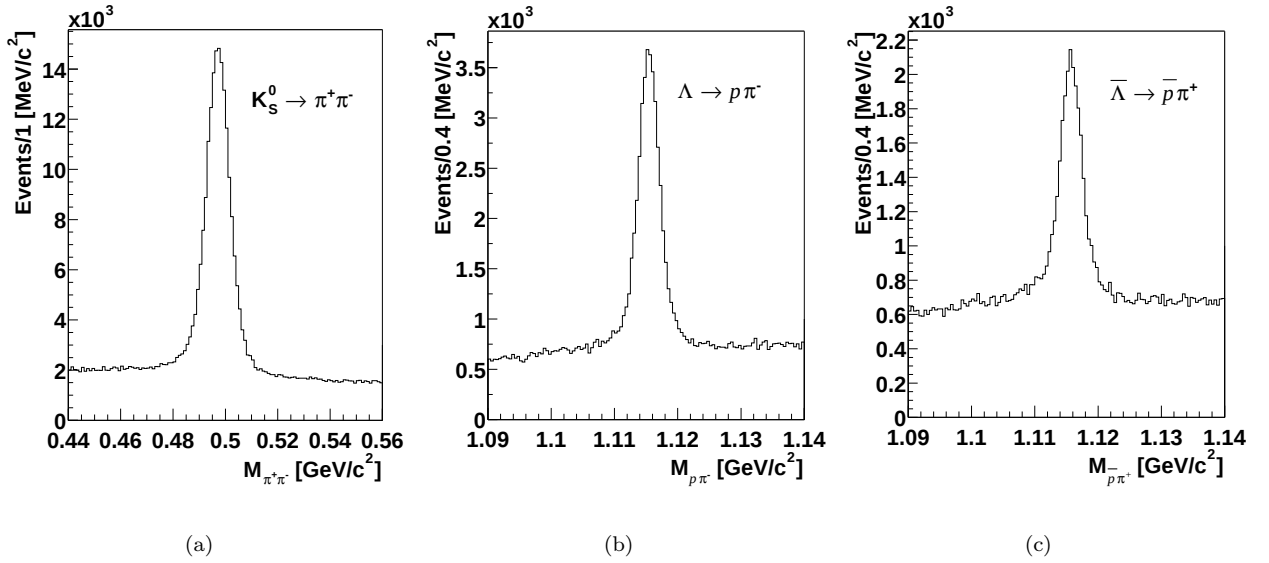
Figure 1: The invariant mass distributions for oppositely charged particle pairs, assuming a) \pi^+\pi^- , b) p\pi^- and c) \bar{p}\pi^+ mass assignments for the carbon target sample after application of the selection criteria described in the text.
