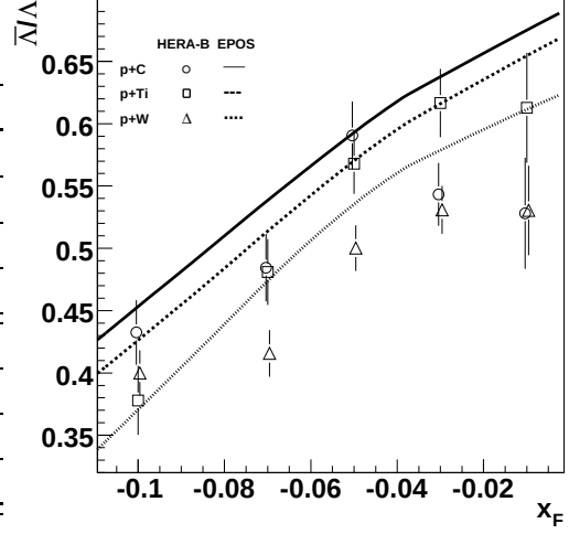
(a) \bar{\Lambda}/\Lambda vs. x_F
