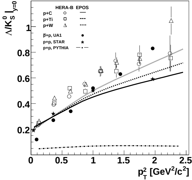
Figure 7: The ratios of \Lambda/K_S^0 vs. p_T^2 at y \sim 0 . The open points show the measured values and the solid points show the results from STAR and UA1 collaborations. The various lines indicate the predictions of PYTHIA and EPOS. The error bars include only statistical contributions.
