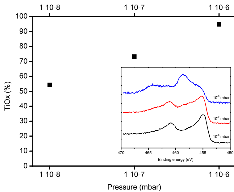
Figure 5. Titanium oxide content in a Ti layer evaporated on a gold substrate under different vacuum pressure. The insert shows the Ti 2p spectra of a 10 nm titanium layer deposited at 10^{-6} , 10^{-7} and 10^{-8} mbar
