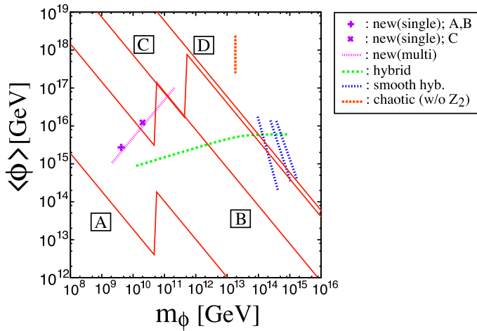
FIG. 1: Constraints from the gravitino production by the inflaton decay, for m_{3/2} = 1 TeV with B_h = 1 (case A), m_{3/2} = 1 TeV with B_h = 10^{-3} (case B), m_{3/2} = 100 TeV (case C), and m_{3/2} = 1 GeV (case D). The region above the solid (red) line is excluded for each case. For m_\phi \gtrsim \Lambda , we used the anomaly-induced inflaton decay into the hidden gauge/gauginos to estimate the gravitino abundance (5), while the gravitino pair production (7) was used for m_\phi \lesssim \Lambda . The typical values of \langle\phi\rangle and m_\phi for the single-field new [23], multi-field new [24], hybrid [11] and smooth hybrid [12], and chaotic [25] inflation models are also shown. Note that we adopt the chaotic inflation model without discrete symmetries, in which case \langle K_\phi \rangle is expected to be around the Planck scale.
