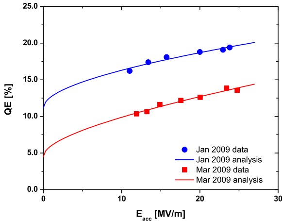
Figure 2: QE vs. accelerating gradient at the cathode for cathode #77.2 obtained at FLASH January 2009 (blue) and March 2009 (red); symbols: data, lines: fit by Eq. 1.
