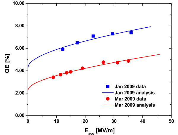
Figure 3: QE vs. accelerating gradient at the cathode for cathode #128.1 obtained at PITZ January 2009 (blue) and March 2009 (red); symbols: data, lines: fit by Eq. 1.
