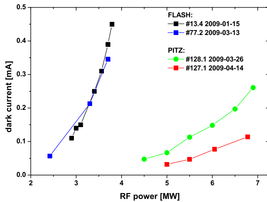
Figure 5: Dark current as function of RF-power for different cathodes measured at FLASH and PITZ.
