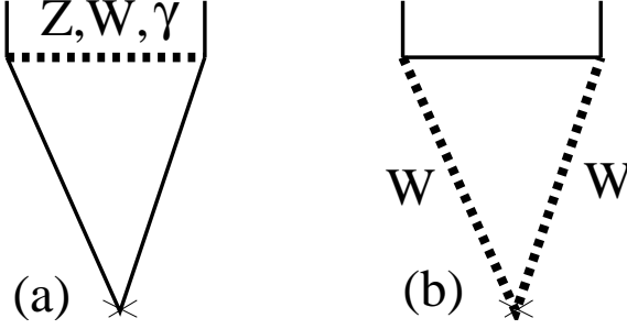
Figure 1: Diagrams, contributing to vertex Zqq (a) and (b). The two-loop diagrams are obtained by attaching one virtual gluon in all possible ways. The case (b) represents nonabelian part, that gives contribution \phi_{NA}(z) in the text. Diagram (a) with W exchange also contributes to \phi_{NA}(z) .
