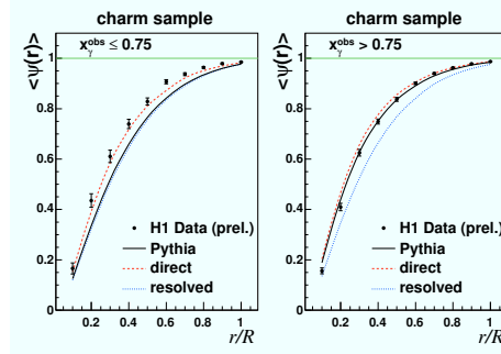
Figure 15. Mean integrated jet shape in charm photoproduction.
