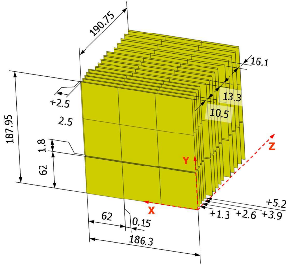
Figure 3. Details of the passive areas and layer offsets. Offsets are indicated by single-headed arrows. All distances are in mm.
