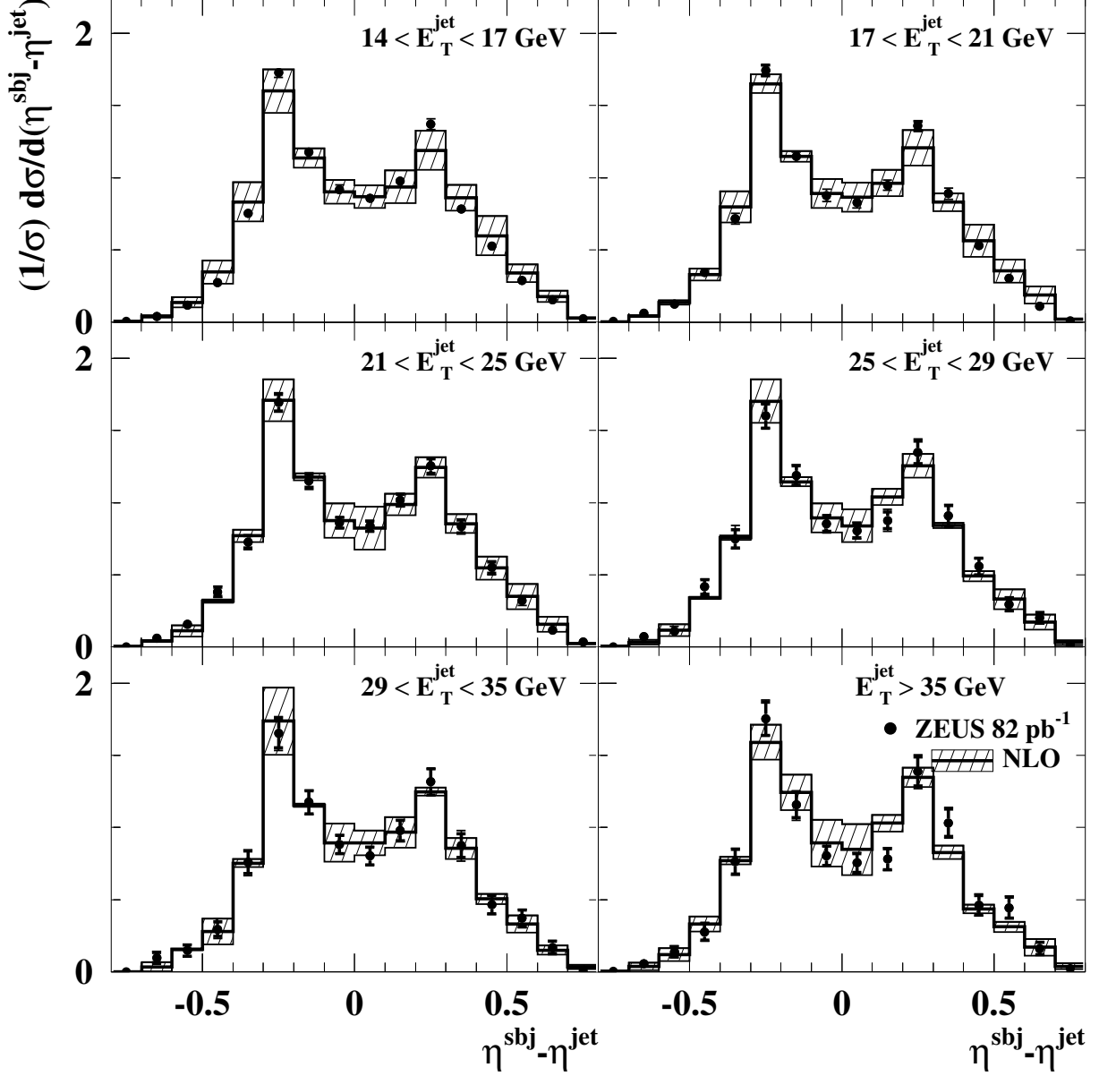
Figure 7: Measured normalised differential subjet cross sections (dots) for jets with E_T^{\text{jet}} > 14 \text{ GeV} and -1 < \eta^{\text{jet}} < 2.5 which have two subjets for y_{\text{cut}} = 0.05 in the kinematic region given by Q^2 > 125 \text{ GeV}^2 as functions of \eta^{\text{subj}} - \eta^{\text{jet}} in different regions of E_T^{\text{jet}} . Other details are as in the caption to Fig. 3.
