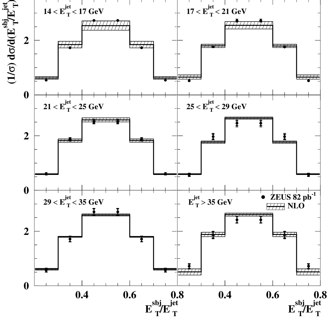
Figure 6: Measured normalised differential subjet cross sections (dots) for jets with E_T^{\text{jet}} > 14 \text{ GeV} and -1 < \eta^{\text{jet}} < 2.5 which have two subjets for y_{\text{cut}} = 0.05 in the kinematic region given by Q^2 > 125 \text{ GeV}^2 as functions of E_T^{\text{sbj}}/E_T^{\text{jet}} in different regions of E_T^{\text{jet}} . Other details are as in the caption to Fig. 3.
