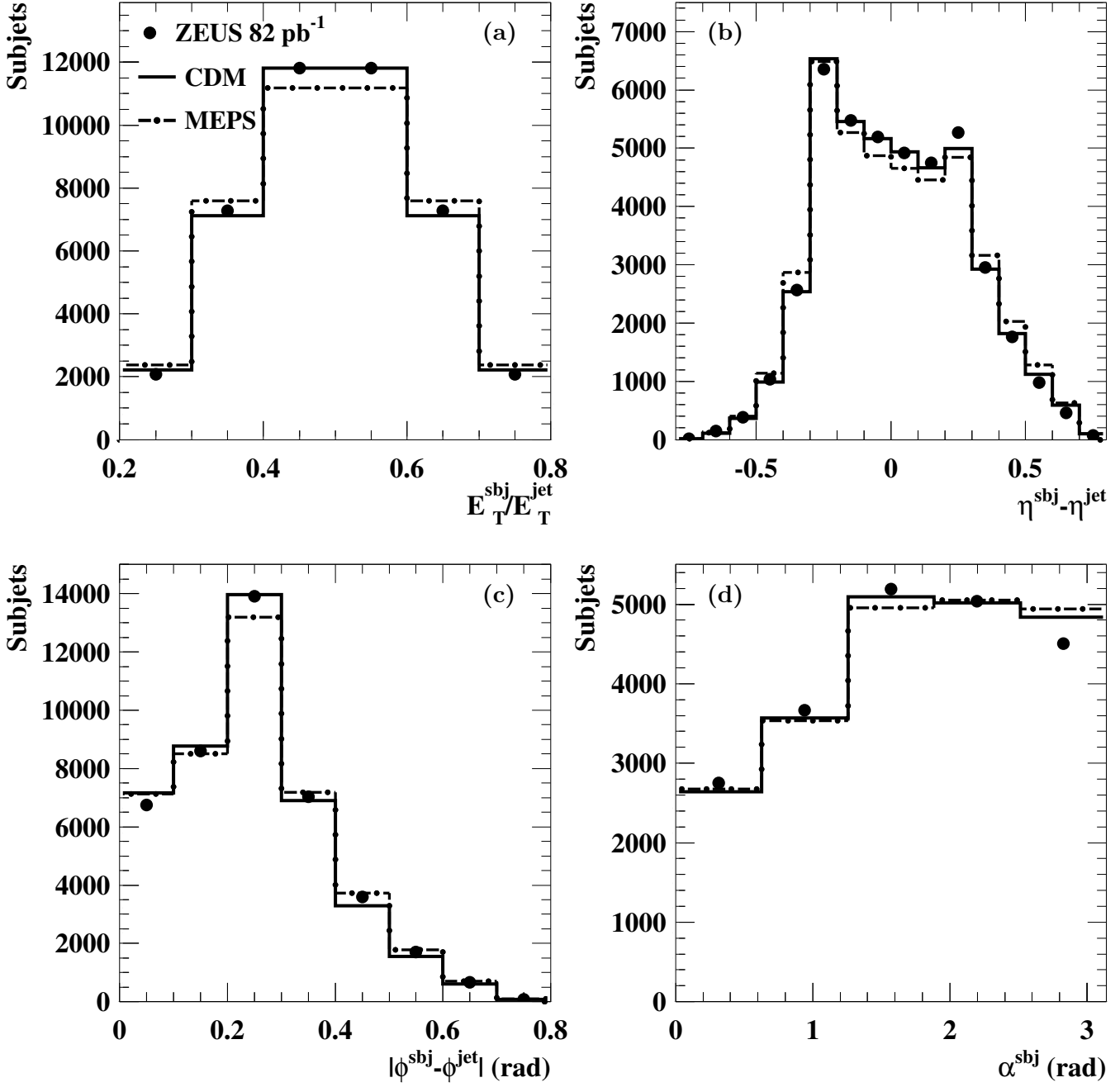
Figure 2: Detector-level normalised subject data distributions (dots) for jets with E_T^{\text{jet}} > 14 GeV and -1 < \eta^{\text{jet}} < 2.5 which have two subjects for y_{\text{cut}} = 0.05 in the kinematic region given by Q^2 > 125 GeV 2 as functions of (a) E_T^{\text{subj}}/E_T^{\text{jet}} , (b) \eta^{\text{subj}} - \eta^{\text{jet}} , (c) |\phi^{\text{subj}} - \phi^{\text{jet}}| and (d) \alpha^{\text{subj}} . The statistical uncertainties are smaller than the marker size. For comparison, the distributions of the CDM (solid histograms) and MEPS (dot-dashed histograms) Monte Carlo models are included.
