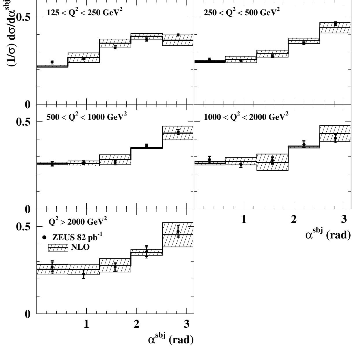
Figure 15: Measured normalised differential subjet cross sections (dots) for jets with E_T^{\text{jet}} > 14 \text{ GeV} and -1 < \eta^{\text{jet}} < 2.5 which have two subjets for y_{\text{cut}} = 0.05 in the kinematic region given by Q^2 > 125 \text{ GeV}^2 as functions of \alpha^{\text{subjet}} in different regions of Q^2 . Other details are as in the caption to Fig. 3.
