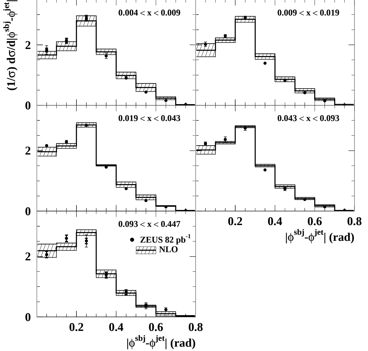
Figure 21: Measured normalised differential subjet cross sections (dots) for jets with E_T^{\text{jet}} > 14 \text{ GeV} and -1 < \eta^{\text{jet}} < 2.5 which have two subjets for y_{\text{cut}} = 0.05 in the kinematic region given by Q^2 > 125 \text{ GeV}^2 as functions of |\phi^{\text{subj}} - \phi^{\text{jet}}| in different regions of x . Other details are as in the caption to Fig. 3.
