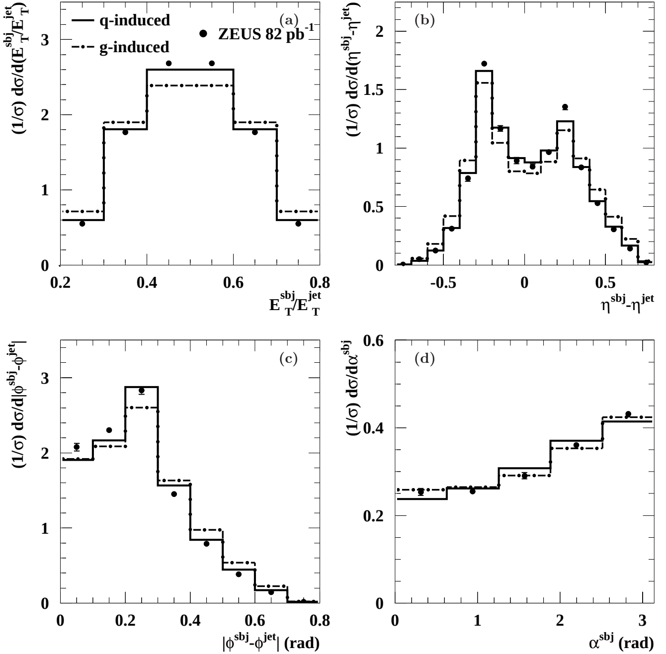
Figure 5: Measured normalised differential subjet cross sections (dots) for jets with E_T^{\text{jet}} > 14 \text{ GeV} and -1 < \eta^{\text{jet}} < 2.5 which have two subjets for y_{\text{cut}} = 0.05 in the kinematic region given by Q^2 > 125 \text{ GeV}^2 as functions of (a) E_T^{\text{subj}}/E_T^{\text{jet}} , (b) \eta^{\text{subj}} - \eta^{\text{jet}} , (c) |\phi^{\text{subj}} - \phi^{\text{jet}}| and (d) \alpha^{\text{subj}} . For comparison, the NLO predictions for quark- (solid histograms) and gluon-induced (dot-dashed histograms) processes are included. Other details are as in the caption to Fig. 3.
