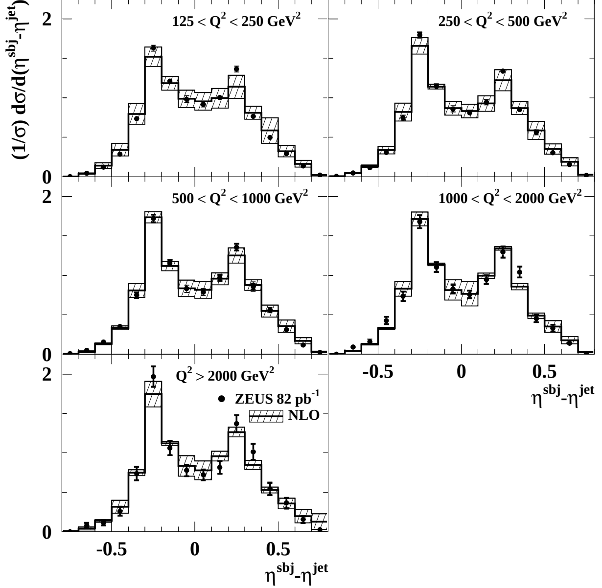
Figure 13: Measured normalised differential subjet cross sections (dots) for jets with E_T^{\text{jet}} > 14 GeV and -1 < \eta^{\text{jet}} < 2.5 which have two subjets for y_{\text{cut}} = 0.05 in the kinematic region given by Q^2 > 125 GeV 2 as functions of \eta^{\text{subj}} - \eta^{\text{jet}} in different regions of Q^2 . Other details are as in the caption to Fig. 3.
