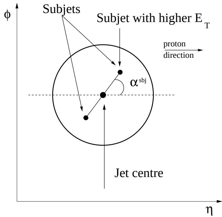
Figure 1: Schematic representation of the \alpha^{\text{sbj}} variable.
