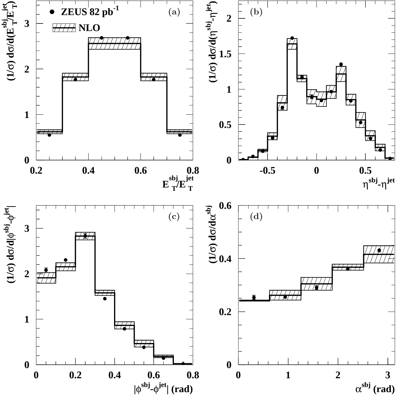
Figure 3: Measured normalised differential subjet cross sections (dots) for jets with E_T^{\text{jet}} > 14 \text{ GeV} and -1 < \eta^{\text{jet}} < 2.5 which have two subjets for y_{\text{cut}} = 0.05 in the kinematic region given by Q^2 > 125 \text{ GeV}^2 as functions of (a) E_T^{\text{subj}}/E_T^{\text{jet}} , (b) \eta^{\text{subj}} - \eta^{\text{jet}} , (c) |\phi^{\text{subj}} - \phi^{\text{jet}}| and (d) \alpha^{\text{subj}} . The inner error bars represent the statistical uncertainties of the data, the outer error bars show the statistical and systematic uncertainties added in quadrature. In many cases, the error bars are smaller than the marker size and are therefore not visible. For comparison, the NLO QCD predictions (solid histograms) are included. The hatched bands represent the theoretical uncertainty.
