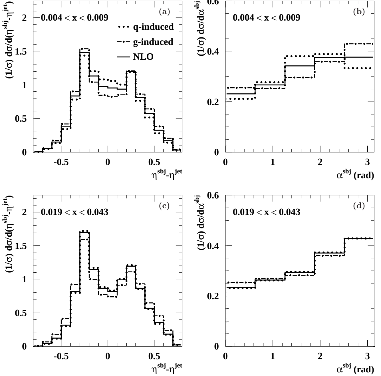
Figure 25: Predicted normalised differential subjet cross sections (solid histograms) for jets with E_T^{\text{jet}} > 14 \text{ GeV} and -1 < \eta^{\text{jet}} < 2.5 which have two subjets for y_{\text{cut}} = 0.05 in the kinematic region given by Q^2 > 125 \text{ GeV}^2 as functions of (a,c) \eta^{\text{subj}} - \eta^{\text{jet}} and (b,d) \alpha^{\text{subj}} in different regions of x . The NLO predictions for quark- (dotted histograms) and gluon-induced (dot-dashed histograms) processes are also shown separately.
