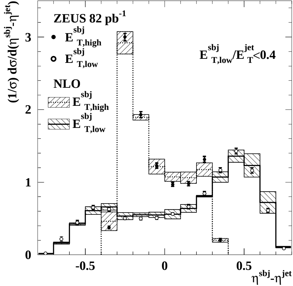
Figure 4: Measured normalised differential subjet cross sections for jets with E_T^{\text{jet}} > 14 \text{ GeV} and -1 < \eta^{\text{jet}} < 2.5 which have two subjets for y_{\text{cut}} = 0.05 in the kinematic region given by Q^2 > 125 \text{ GeV}^2 and E_{T,\text{low}}^{\text{sbj}}/E_T^{\text{jet}} < 0.4 as functions of \eta^{\text{sbj}} - \eta^{\text{jet}} separately for the higher (dots) and lower (open circles) E_T^{\text{sbj}} subjets. Other details are as in the caption to Fig. 3.
