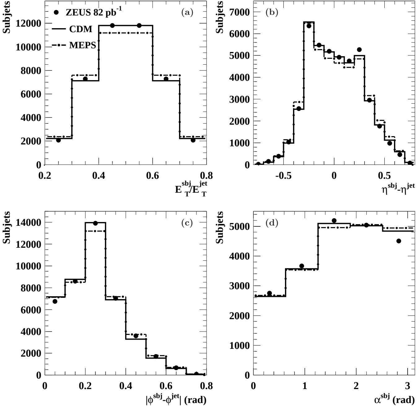
Figure 2: Detector-level normalised subject data distributions (dots) for jets with E_T^{\text{jet}} > 14 \text{ GeV} and -1 < \eta^{\text{jet}} < 2.5 which have two subjects for y_{\text{cut}} = 0.05 in the kinematic region given by Q^2 > 125 \text{ GeV}^2 as functions of (a) E_T^{\text{subj}}/E_T^{\text{jet}} , (b) \eta^{\text{subj}} - \eta^{\text{jet}} , (c) |\phi^{\text{subj}} - \phi^{\text{jet}}| and (d) \alpha^{\text{subj}} . The statistical uncertainties are smaller than the marker size. For comparison, the distributions of the CDM (solid histograms) and MEPS (dot-dashed histograms) Monte Carlo models are included.
