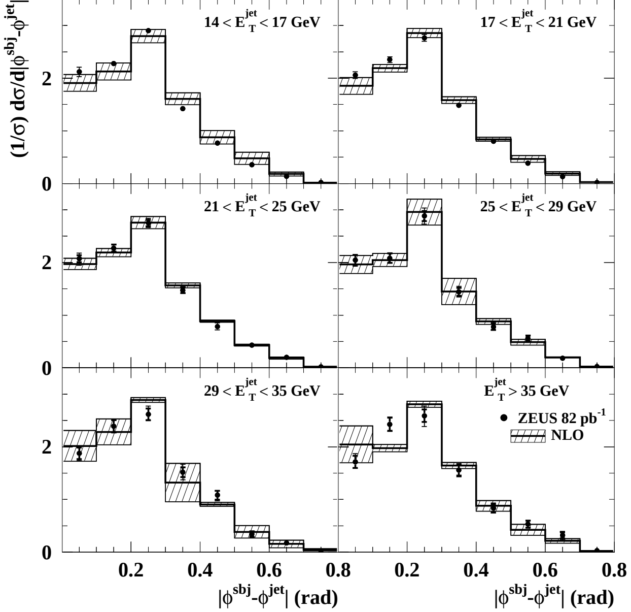
Figure 8: Measured normalised differential subjet cross sections (dots) for jets with E_T^{\text{jet}} > 14 \text{ GeV} and -1 < \eta^{\text{jet}} < 2.5 which have two subjets for y_{\text{cut}} = 0.05 in the kinematic region given by Q^2 > 125 \text{ GeV}^2 as functions of |\phi^{\text{subj}} - \phi^{\text{jet}}| in different regions of E_T^{\text{jet}} . Other details are as in the caption to Fig. 3.
