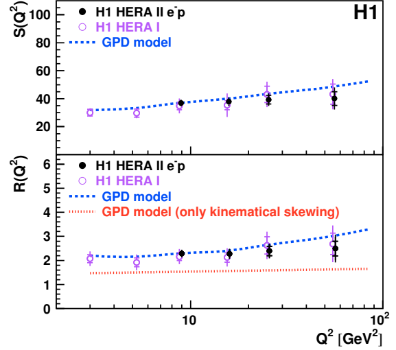
Figure 7. The observables S and R as a function of Q^2 . The dashed curves show the predictions of the GPD models. The dotted curve shows the prediction of a GPD model based on an approximation where only the kinematical part of the skewing is taken into account.
