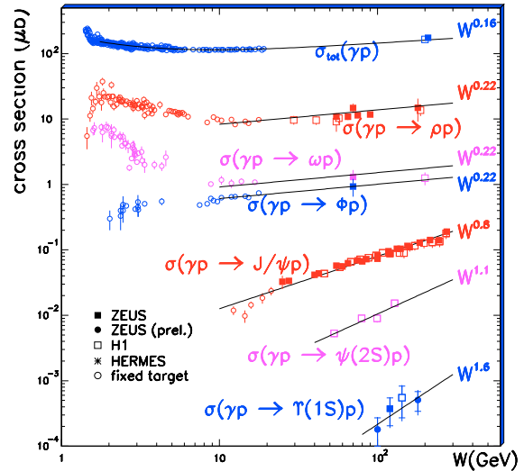
Figure 1. Cross sections as a function of W of the elastic photoproduction of \rho , \omega , \phi , J/\Psi , \Psi' and \Upsilon vector mesons. The solid lines represent fits of the W^\delta dependence.
