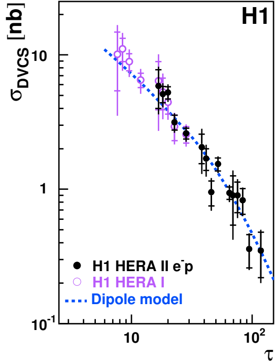
Figure 8. DVCS cross section as a function of the scaling variable \tau = Q^2/Q_s^2(x) . The dashed curves represent predictions of the dipole model [21,17].
