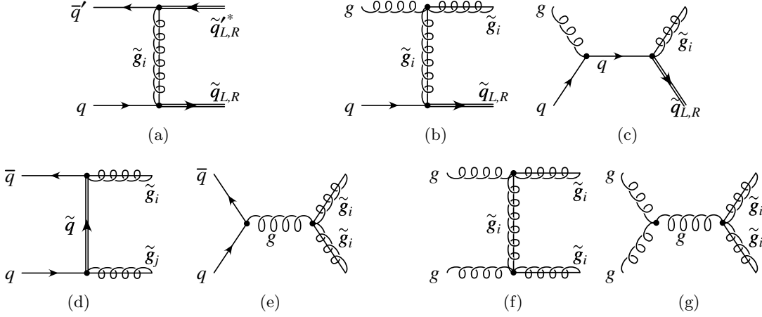
FIG. 4: Feynman diagrams for different-flavor squark production in quark annihilation (a), squark-gluino production (b,c), gluino production in quark annihilation (d,e) and gluino production in gluon fusion (f,g). [The indices i, j count the two gluinos in the N=2 hybrid model, and should be ignored for the N=1 MSSM.]
