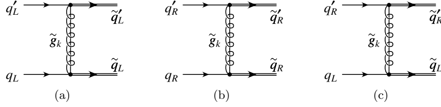
FIG. 1: Feynman diagrams for squark production of different flavors at hadron colliders. [The index k counts the two gluinos in the N=2 hybrid model, to be ignored for the N=1 MSSM.]
