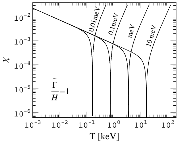
FIG. 1: Isocontours of \tilde{\Gamma}/H = 1 for different \gamma' masses.
