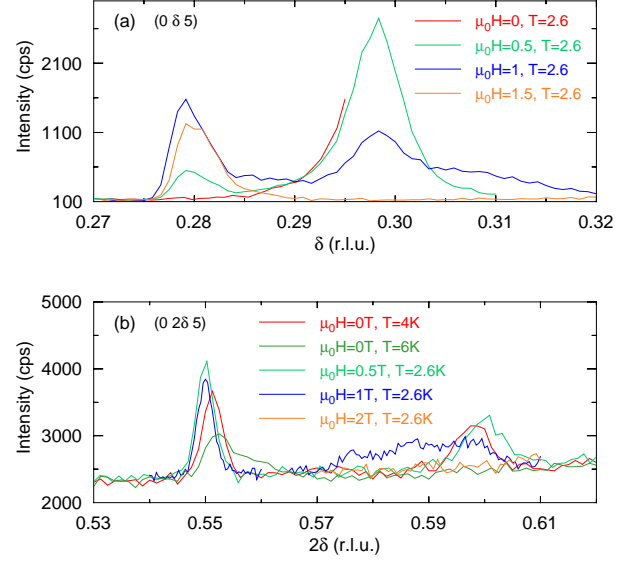
FIG. 13: (Color online) k-scans over (a) (0, \delta, 5) and (b) (0, 2\delta, 5) positions as function of magnetic field H_{\parallel b} and temperature below T_N^{Tb} .
