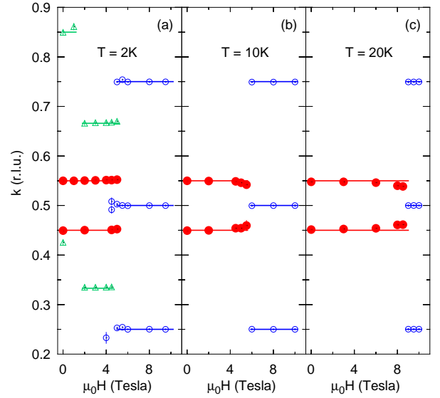
FIG. 8: (Color online) Incommensurability \delta of the superlattice reflections (0, 2\delta^{Mn}, 4) and (0, 1-2\delta^{Mn}, 4) below H_C^b (closed circles) and (0, 0.25, 4) , (0, 0.5, 4) and (0, 0.75, 4) above H_C^b (open circles), measured at (a) T = 2 K, (b) T = 10 K and (c) T = 20 K as function of magnetic field H||b . At T = 2 K in addition (0, \delta^{Tb}, 5) and (0, 2\delta^{Tb}, 5) reflections are shown below and above H_C^{Tb} (open triangles).
