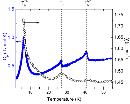
FIG. 1: (Color online) Temperature dependence of the specific heat ( C_p ) and magnetic susceptibility \chi of a small single crystal from the TbMnO 3 boule. For the magnetization measurements a field of 0.01 T was applied along the c -axis. The C_p(T) and \chi(T) data indicate three successive phase transitions at 7 K, 27 K and 41 K corresponding to T_N^{Tb} , T_s , T_N^{Mn} , respectively.
