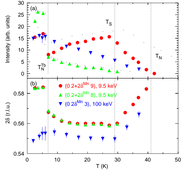
FIG. 2: (Color online) Temperature dependence at zero field and 9.5 keV photon energy of the (a) intensity and (b) k -component of the wave vector of the A-mode (0, 2+2\delta^{Mn}, 9) and F-mode (0, 2+2\delta^{Mn}, 8) reflections. The respective temperatures T_N , T_s and T_N^{Tb} are indicated by dashed lines. In addition data for the A-mode (0, 2\delta^{Mn}, 3) reflection measured at 100 keV are plotted. Due to a systematic offset the absolute wave numbers are not accurate.
