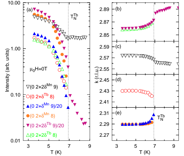
FIG. 4: (Color online) Temperature dependence of (a) intensities and (b-e) wave number of the first and second harmonic structural Mn- and Tb-superlattice reflections in the Tb ordered phase T < T_N^{Tb} at zero field.
