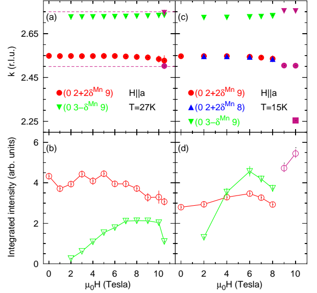
FIG. 5: (Color online) Magnetic field dependence of (a) wave vector and (b) intensity of the second harmonic (0, 2+2\delta^{Mn} , 9) (circles) and first harmonic (0, 3-\delta^{Mn} , 9) (triangles) superlattice reflection at a sample temperature of T = 27 K for H||a . Magnetic field dependence of (c) wave vector and (d) intensities of the CM and IC superlattice reflection for magnetic field H||a at a sample temperature T = 15 K. At \mu_0 H_C^a = 9 T the reflections lock in at CM positions. The horizontal dashed lines show the half and quarter integer positions of the CM first and second harmonic reflections above H_C^a .
