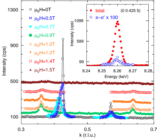
FIG. 7: (Color online) K-scans of the (0, \delta^{Tb}, 5) and (0, 1-\delta^{Tb}, 5) reflection as function of field H||a at a sample temperature T = 4 K without polarization analysis. The inset shows an energy scan over the Tb L_2 absorption edge with and without polarization analysis in the \pi - \sigma' channel. The total signal only shows the resonant intensity. The fluorescence background is subtracted using an energy scan performed off the reflection position.
