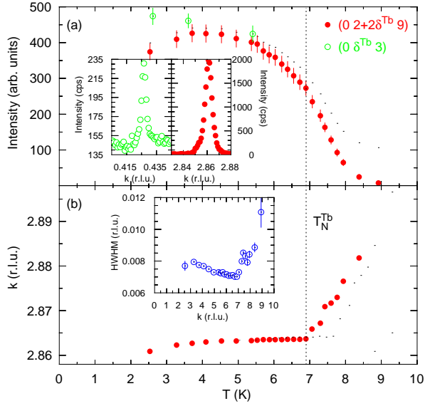
FIG. 3: (Color online) Tb superlattice reflection as function of temperature. (a) shows the intensity of the (0, 2+2\delta^{Tb}, 9) and the (0, \delta^{Tb}, 3) . (b) shows the variation of the propagation vector of the (0, 2+2\delta^{Tb}, 9) superlattice reflection. In the inset, a scan over the first and second harmonic peak along the b^* -direction is shown.
