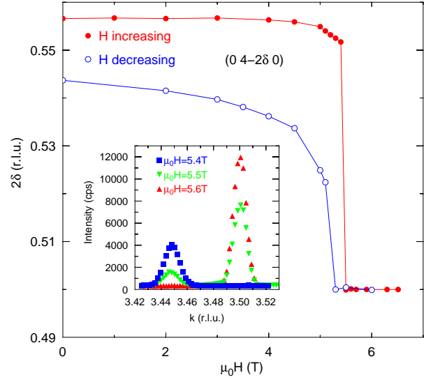
FIG. 10: (Color online) Hysteresis of the superlattice reflections measured at T = 10 K. Solid circles show the data measured with increasing field, open circles the data measured with decreasing field. The inset shows the superlattice reflections at the phase transition for increasing field.
