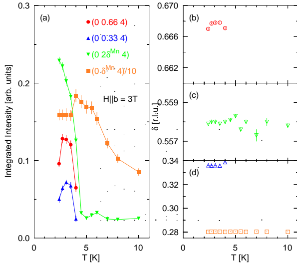
FIG. 12: (Color online) (a) Temperature dependence of the intensities of the Mn and Tb first and second harmonic superlattice reflections measured at magnetic field \mu_0 H = 3 T. (b) shows the corresponding k-components of the wave vector. The measurement is performed by going from the intermediate Tb ordered phase through T_N^{Tb} into the purely Mn ordered phase.
