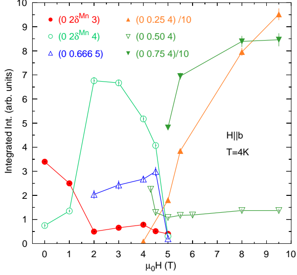
FIG. 11: (Color online) Intensities of the (0\ 0.55\ 3) , (0\ 0.55\ 4) , and (0\ 0.66\ 5) reflections below H_C^b and (0\ 0.25\ 4) and (0\ 0.5\ 4) above H_C^b as function of magnetic field H_{\parallel b} measured at a sample temperature of T = 4 K.
