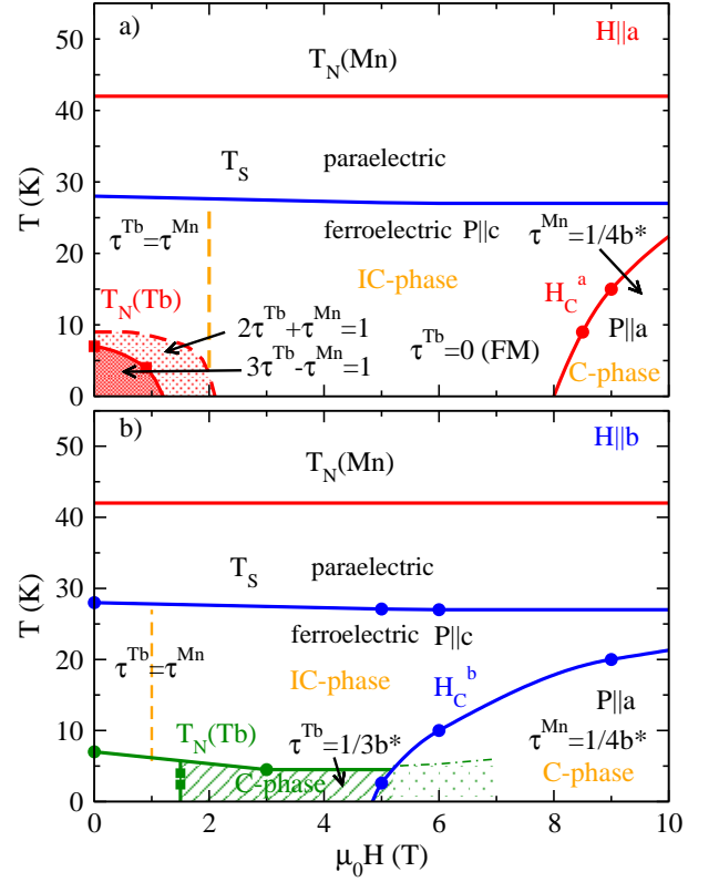
FIG. 15: (Color online) Phase diagram of \text{TbMnO}_3 for fields (a) H \parallel a and (b) H \parallel b . In (a) the light shaded area represents the intermediate phase region and the dark shaded area the Tb AF ordered state found for field H \parallel a . In (b) the green line represents T_N^{Tb} as found for magnetic field H \parallel b . The green shaded area shows the intermediate CM Tb ordered phase for H \parallel b . The IC to CM transition for the manganese order is shown for H \parallel a and H \parallel b . The vertical dashed line defines the onset of the first harmonic reflections.
