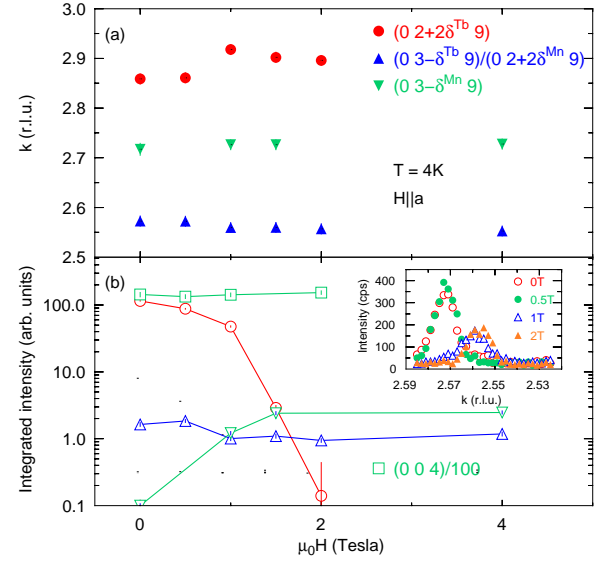
FIG. 6: (Color online) Field dependence at T = 4 K of the terbium and manganese superlattice reflections with magnetic field H\parallel a . (a) peak positions (closed symbols) and (b) the corresponding intensities (open symbols) are shown. Open rectangles show the (0, 0, 4) main Bragg intensity divided by a factor 100. The inset in (b) shows the peak profiles of the (0, 3-\delta^{Tb}, 9) and (0, 2+2\delta^{Tb}, 9) reflections for different fields.
