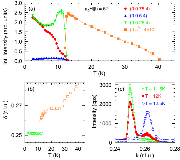
FIG. 14: (Color online) (a) Intensity behavior of CM and IC superlattice reflections measured at H = 6 T below (CM) and above (IC) the critical temperature. (b) Corresponding wave number \delta^{Mn} as function of temperature for the first harmonic F-mode reflection. (c) k-scans in the region of coexistence of the CM and IC phase at the critical temperature.
