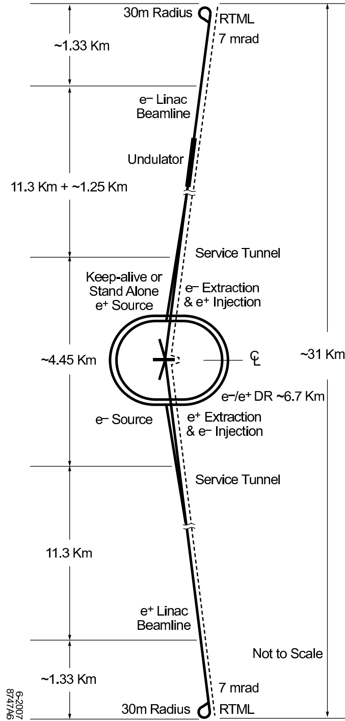
Figure 2.3: Schematic layout of the ILC complex for 500 GeV centre-of-mass energy [38]
