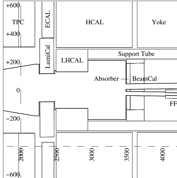
Figure 6.2: Forward region of the simulated detector geometry, compressed by a factor of 2 in z -direction (values are given in millimetres)
