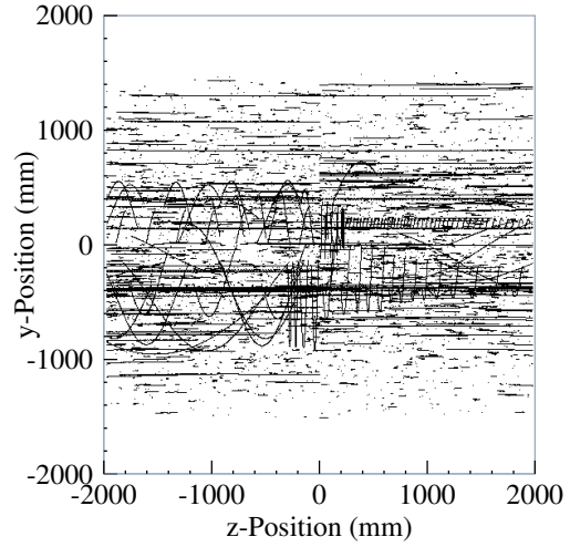
Figure 7.37: Mokka hits in the TPC from 100 bunch crossings, seen from the side. This view reveals the peculiar structure of the microcurlers.
