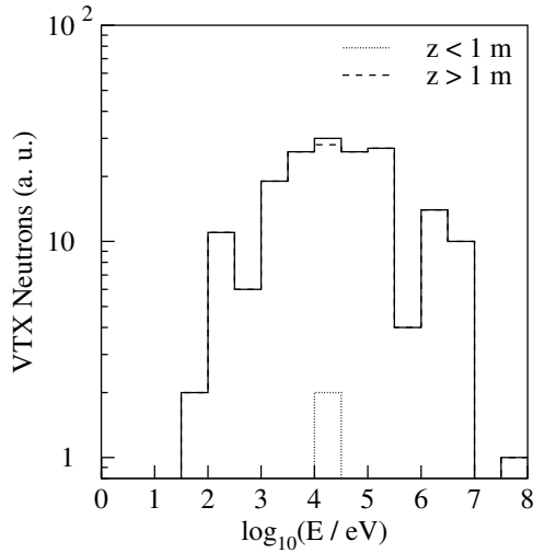
Figure 7.64: Energy distribution of neutrons traversing the vertex detector, using the physics list LHEP_BERT_HP
