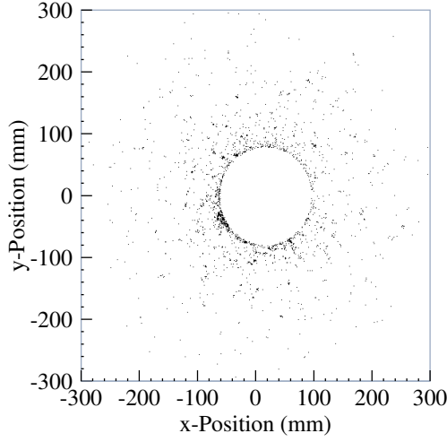
Figure 7.59: Backscattering sources in the LumiCal for an inner radius of 80 mm, front view. The LumiCal is not a significant source of backscattering particles.
