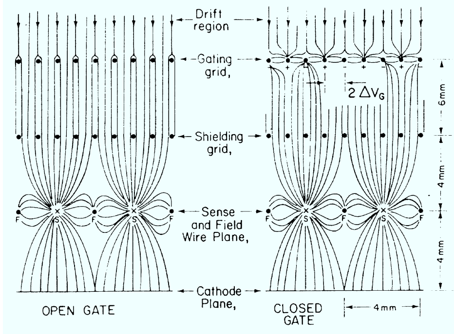
Figure 5.10: Working principle of gating wires, here shown for a drift chamber with wire amplification [99]. The open gate (left) does not influence the drifting electrons, whereas the closed gate (right) blocks the path for back-drifting ions.
