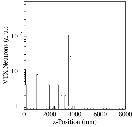
Figure 7.18: Origins of neutrons traversing the vertex detector
