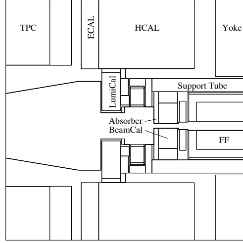
Figure 7.50: Simulated forward region according to the improved layout of 2004 (compressed by a factor of 2 in z -direction)
