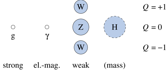
Figure 1.2: Bosons in the Standard Model. The gluon (g) and the photon ( \gamma ) are massless, whereas the W and the Z bosons acquire their large masses of 80.4 and 91.2 GeV through interaction with the (yet undiscovered) Higgs boson. The gluon is electrically neutral, but it carries colour charge.
