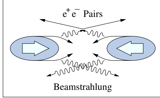
Figure 3.1: Illustration of the pinch effect in bunch collisions. The particles of one bunch are attracted by the electric space charge of the other and emit photons due to their deflection. Those photons can in turn scatter to produce electron-positron pairs.
