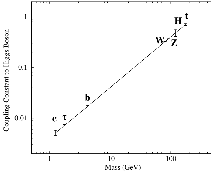
Figure 2.2: The relation between the Higgs coupling constants and the particle masses as they could be determined from high-precision ILC measurements [29]. If the couplings are proportional to the particles’ masses, this would prove that the Higgs mechanism is responsible for the generation of mass, as predicted by the Standard Model.
