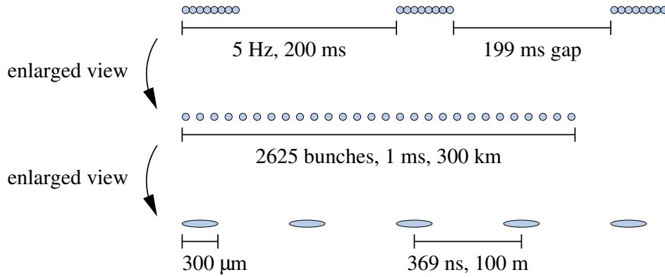
Figure 2.4: Bunch structure of the ILC: 2625 bunches with 2 \cdot 10^{10} particles per bunch form a so-called bunch train of about 1 ms length. Trains are accelerated at a repetition rate of 5 Hz.
