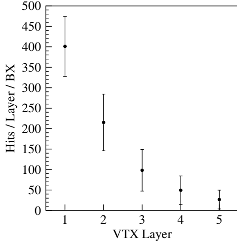
Figure 7.3: Hits on the vertex detector per bunch crossing, in absolute numbers
