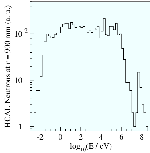
Figure 7.47: Energy distribution of neutrons in the HCAL endcap at r = 900 mm
