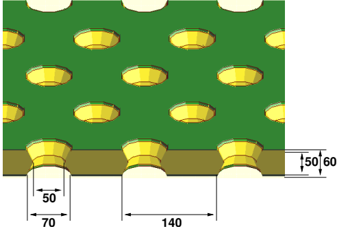
Figure 5.4: Geometry of a standard CERN GEM (values are given in micrometres)
