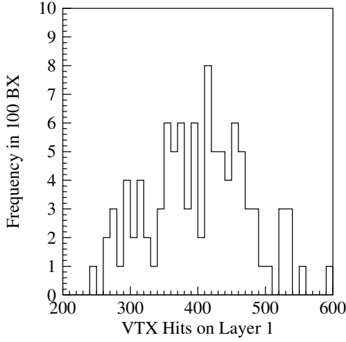
Figure 7.1: Distribution of the number of hits on the innermost layer (layer 1) of the vertex detector
