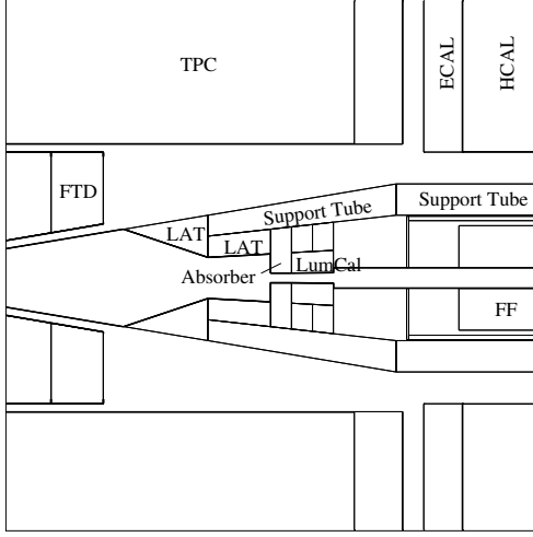
Figure 7.49: Simulated forward region according to the TESLA TDR (compressed by a factor of 2 in z -direction)
