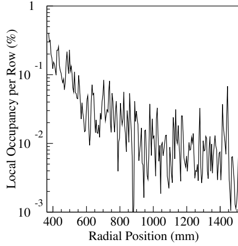
Figure 7.43: Local relative occupancy per pad row in dependency of the radial position (overlay of 100 bunch crossings)
