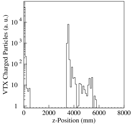
Figure 7.12: Origins of electrons and positrons traversing the vertex detector
