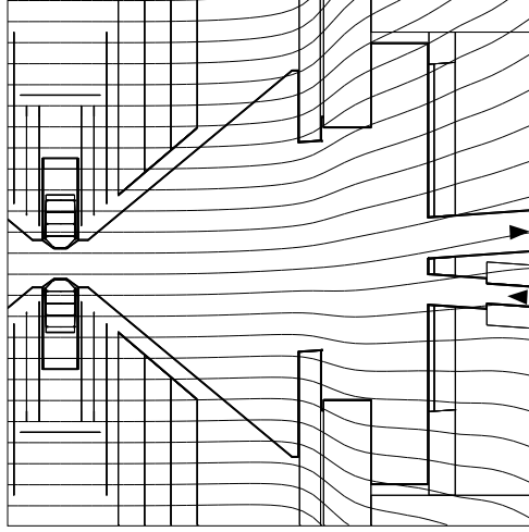
Figure 6.5: Forward region, compressed by a factor of 10 in z -direction. The magnetic field lines of an anti-DID field configuration [116] are superimposed.
