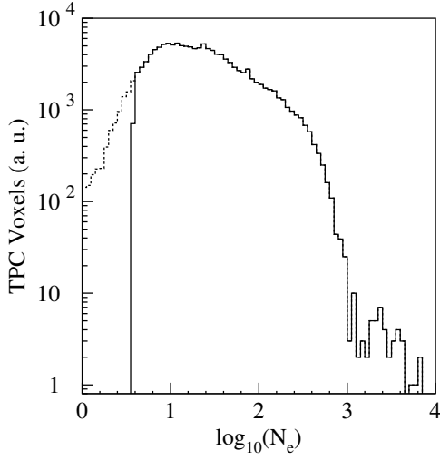
Figure 7.44: Distribution of the primary charge per non-empty voxel. The rising edge corresponds to an assumed electronics threshold of four primary electrons per voxel.
