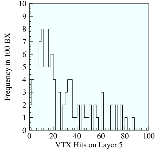
Figure 7.2: Distribution of the number of hits on the outermost layer (layer 5) of the vertex detector
