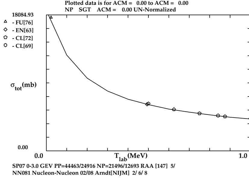
Figure 7.35: Measured total cross-section (“SGT”) for neutron-proton scattering at 0 \text{ MeV} < T_{\text{lab}} < 1 \text{ MeV} , generated by [145]. The measured points are taken from [146]. The vertical axis ranges from 0 barn to approximately 18 barn.
