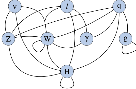
Figure 1.3: Interactions in the Standard Model, represented by possible couplings between the particles (adapted from [8]). The loops indicate self-couplings.
