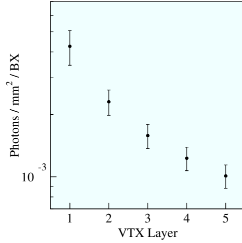
Figure 7.15: Photons traversing the vertex detector per bunch crossing, normalised per unit area
