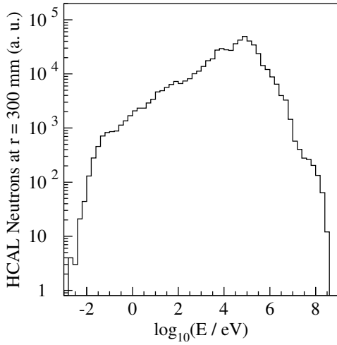
Figure 7.46: Energy distribution of neutrons in the HCAL endcap at r = 300 mm
