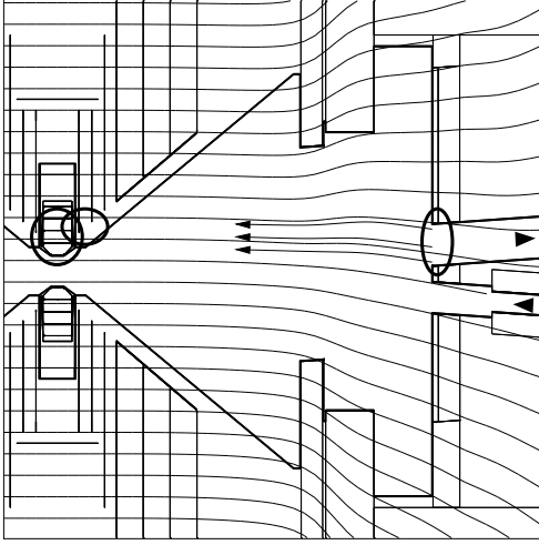
Figure 7.53: Forward region, compressed by a factor of 10 in z -direction. The magnetic field lines of a DID field configuration [153] are superimposed. Backscatterers from the BeamCal are guided into the FTDs and the vertex detector.
