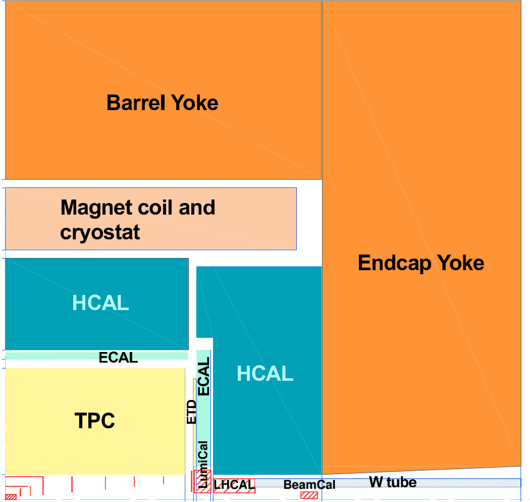
Figure 4.1: Quadrant of the Large Detector Concept [39]
