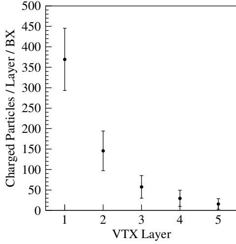
Figure 7.10: Electrons and positrons traversing the vertex detector per bunch crossing, in absolute numbers
