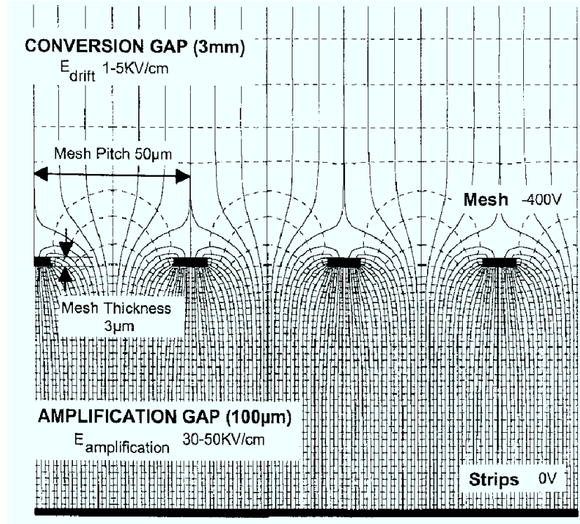
Figure 5.8: Geometry of a Micromegas [95]
