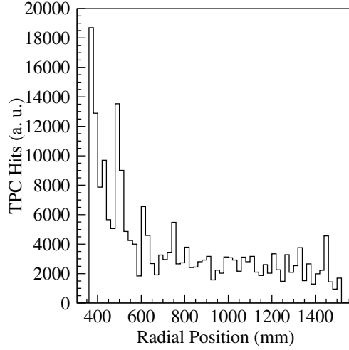
Figure 7.38: Radial distribution of hits in the TPC
