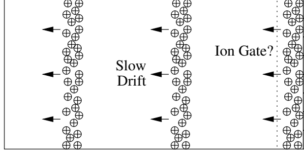
Figure 5.9: Ions that can escape from the amplification system drift back through the chamber volume. Since their drift velocity is so small, they form multiple thin discs that originate from different bunch trains.
