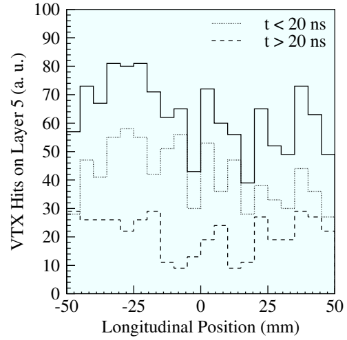
Figure 7.9: Longitudinal distribution of hits on layer 5 of the vertex detector.
