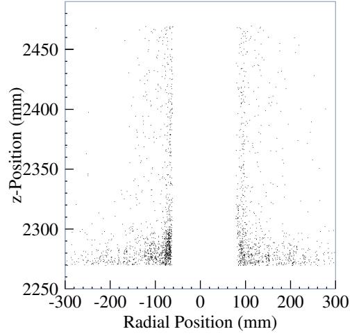
Figure 7.60: Backscattering sources in the LumiCal for an inner radius of 80 mm, top view
