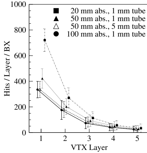
Figure 7.63: Hits on the vertex detector per bunch crossing for different thicknesses of the BeamCal absorber and the beam tube inside the BeamCal
