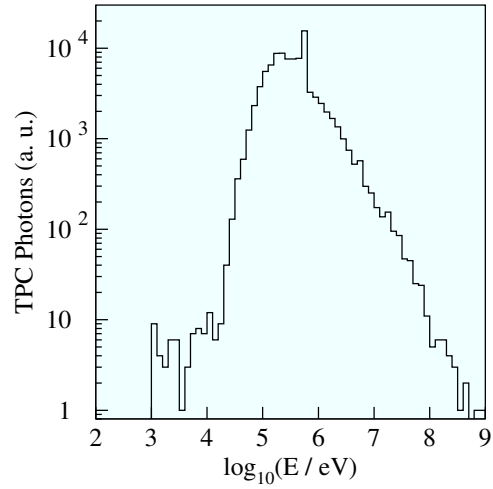
Figure 7.31: Energy distribution of photons that enter the TPC volume
