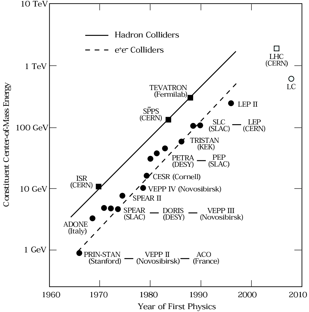
Figure 2.1: The so-called Livingston plot, adapted from [27, 28]: a history of hadron and lepton colliders, indicating an exponential increase of the available centre-of-mass energy in the course of time in the past, similar to Moore’s law of computing power. At the time of the drawing of this plot, the LHC was still believed to deliver first physics around 2005, and the subsequent lepton collider was foreseen for 2008. The former project is slightly delayed, the latter significantly. In any case, the progress of accelerator development seems to have slowed down in the recent years.
