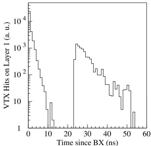
Figure 7.5: Time distribution of hits on layer 1 of the vertex detector.
