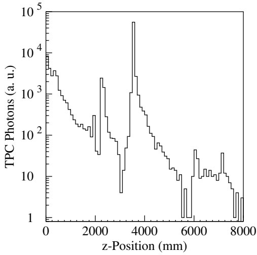
Figure 7.30: Origins of photons that enter the TPC volume
