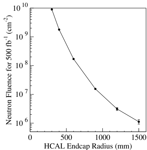
Figure 7.48: Total neutron fluence for 500 fb -1 in the HCAL endcaps, in dependency of the radial position. The upper boundary corresponds to the critical fluence of 10 10 neutrons/cm 2 .
