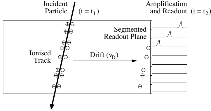
Figure 5.2: Basic principle of a TPC. The position of the track can be reconstructed from the drift time \Delta t = t_2 - t_1 and the drift velocity v_D .
