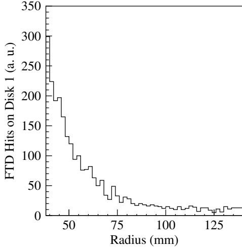
Figure 7.25: Radial distribution of hits on the Forward Tracking Discs
