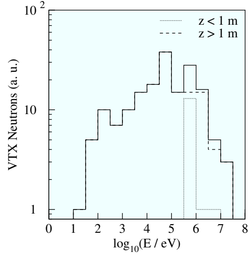
Figure 7.19: Energy distribution of neutrons traversing the vertex detector
