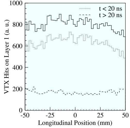
Figure 7.7: Longitudinal distribution of hits on layer 1 of the vertex detector.
