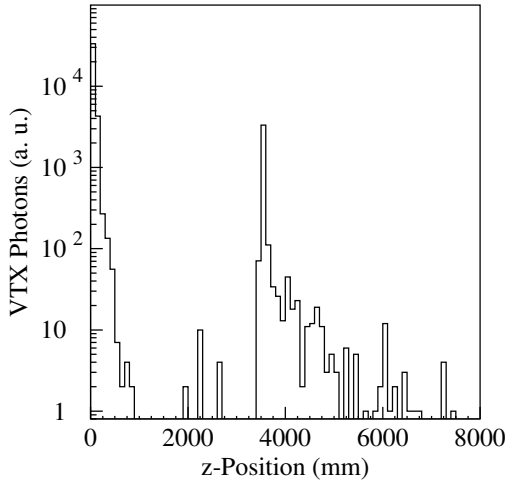
Figure 7.16: Origins of photons traversing the vertex detector
