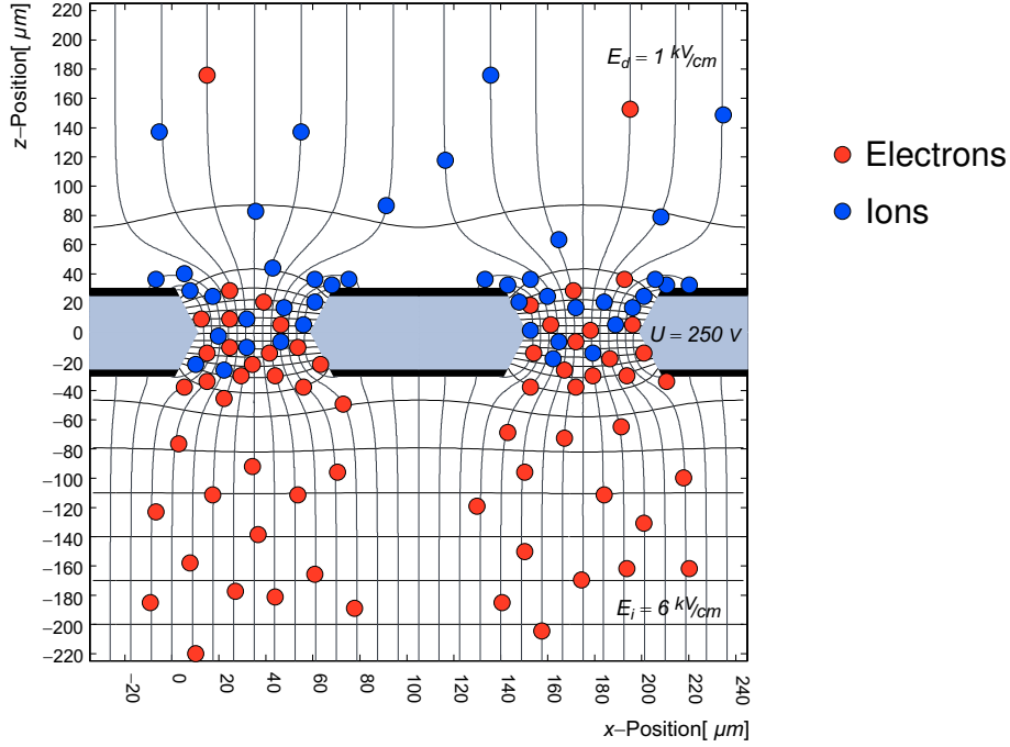
Figure 5.6: Working principle of a GEM foil (adapted from [93])
