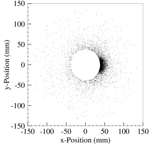
Figure 7.56: Hits on the innermost Forward Tracking Disc in the case of a DID field configuration. The stream of backscattered particles from the BeamCal has an offset from the z -axis and causes a hot spot on the disc.
