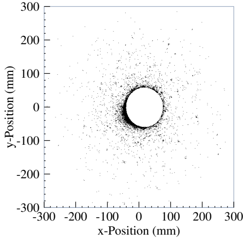
Figure 7.61: Backscattering sources in the LumiCal for an inner radius of 60 mm, front view. The inner surface of the LumiCal gets struck by particles and forms a region of high activity.
