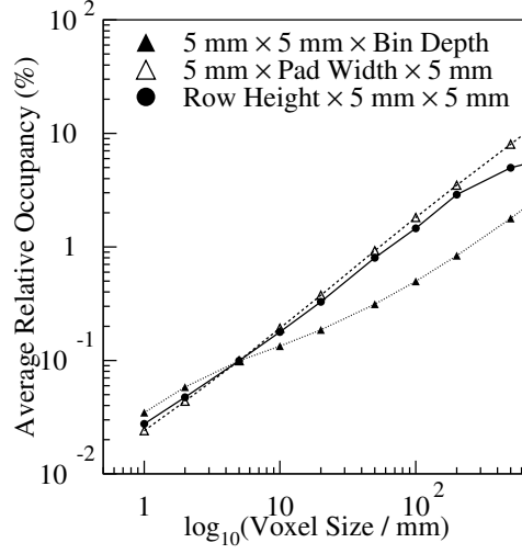
Figure 7.41: The relative occupancy for varying voxel sizes in three dimensions (overlay of 100 bunch crossings)
