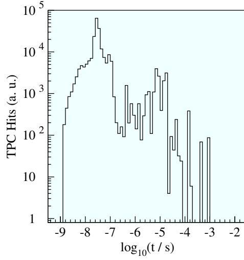
Figure 7.40: Time distribution of hits in the TPC. Note that the double-logarithmic scale ranges from the order of nanoseconds to several milliseconds.
