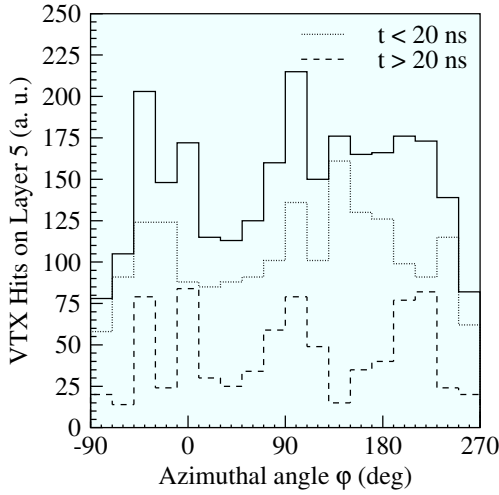
Figure 7.8: Azimuthal distribution of hits on layer 5 of the vertex detector.
