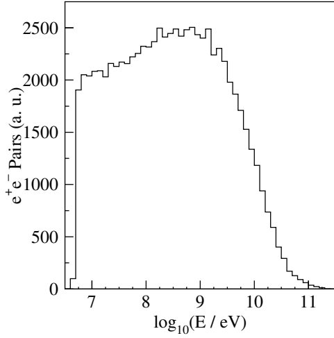
Figure 3.2: Energy spectrum of electron-positron pairs simulated with Guinea-Pig (section 6.1) for nominal beam parameters. The lower edge at 5 MeV corresponds to a momentum cut-off in the simulation.
