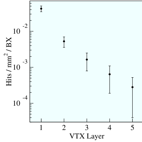
Figure 7.4: Hits on the vertex detector per bunch crossing, normalised per unit area
