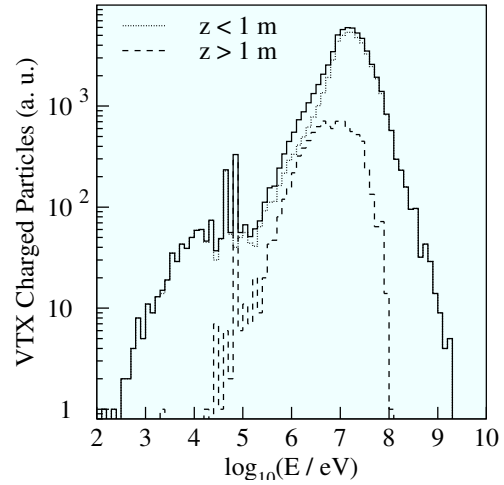
Figure 7.13: Energy distribution of electrons and positrons traversing the vertex detector
