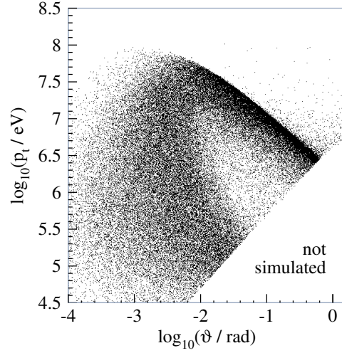
Figure 3.3: Transverse momentum of pairs vs. their polar angle. The void region in the lower right is caused by a momentum cut-off in the simulation. Particles in the upper dark band must be kept away from the vertex detector, but hits from the few particles that have even larger angles and momenta cannot be avoided [56].
