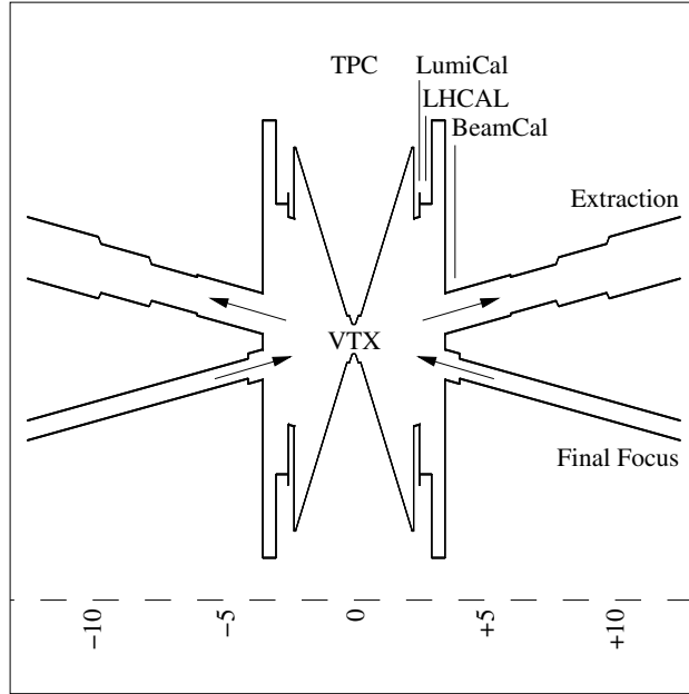
Figure 6.3: Geometry of the simulated beam tube in the xz -plane, compressed by a factor of 40 in z -direction (values are given in metres)
