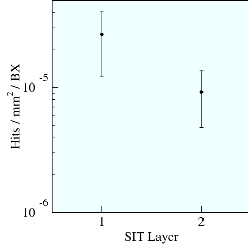
Figure 7.22: Hits on the Silicon Intermediate Tracker per bunch crossing, normalised per unit area
