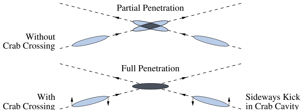
Figure 2.5: Sketch of the crab crossing technique. The crossing angle is greatly exaggerated, but the oblong shape of the bunches is under-exaggerated as well – the actual detriment caused by the crossing angle is similar to what this sketch may suggest.
