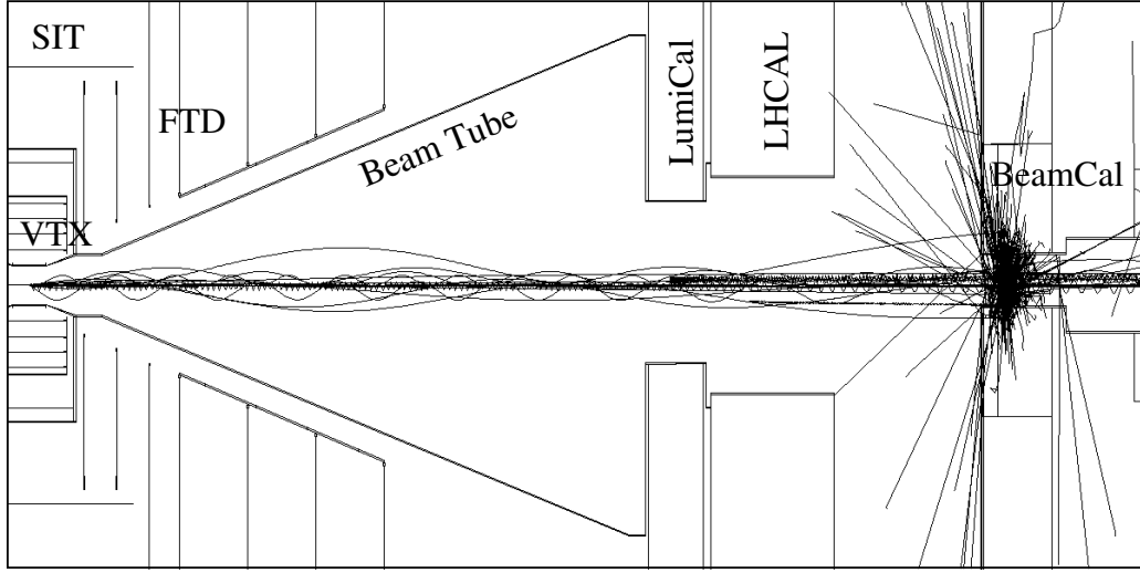
Figure 3.5: Twenty random particles from electron-positron pairs inside the detector (compressed by a factor of 5 in z -direction). Most particles are confined to a tight cone in which they curl around the magnetic field lines and hit the BeamCal. Only few particles (none of the ones shown here) can reach the LumiCal or even the vertex detector and other parts of the detector directly.
