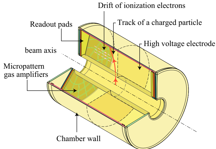
Figure 5.1: Schematic layout of a TPC [39]
