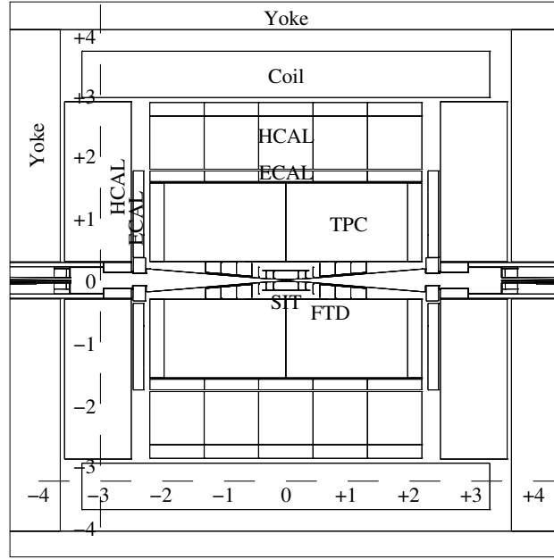
Figure 6.1: Central region of the simulated detector geometry (values are given in metres)
