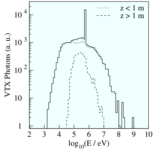
Figure 7.17: Energy distribution of photons traversing the vertex detector
