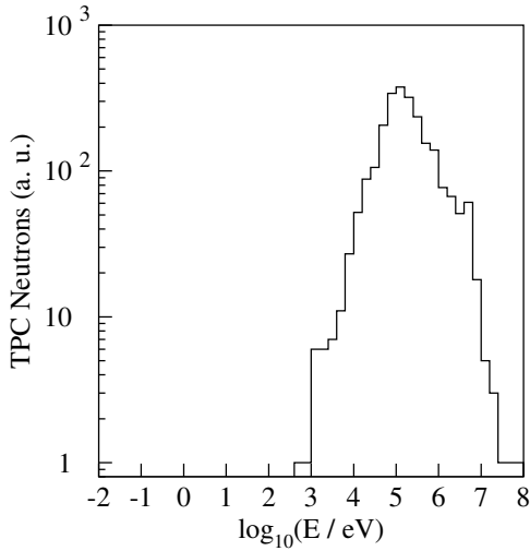
Figure 7.28: Energy distribution of neutrons that enter the TPC volume, at their point of origin
