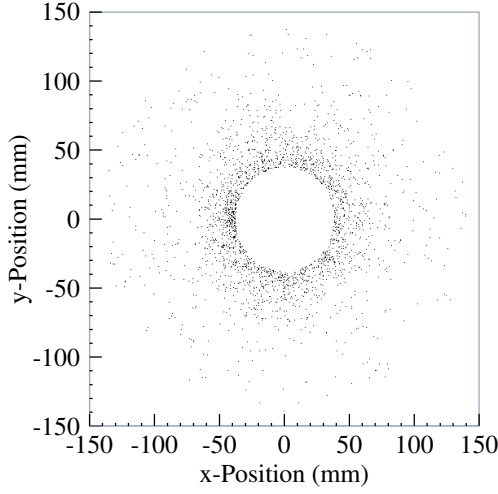
Figure 7.55: Hits on the innermost Forward Tracking Disc in the case of an anti-DID field configuration. Backscattered particles from the BeamCal are mostly guided through the centre of the disc without hitting the detector.
