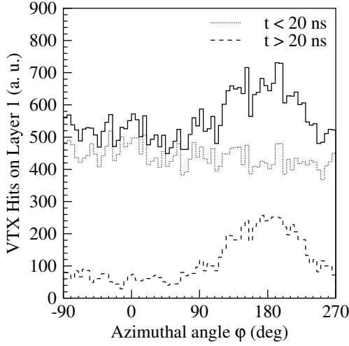
Figure 7.6: Azimuthal distribution of hits on layer 1 of the vertex detector. \varphi = 0 corresponds to the direction of the outgoing beam, \varphi = 180^\circ corresponds to the direction of the incoming beam.
