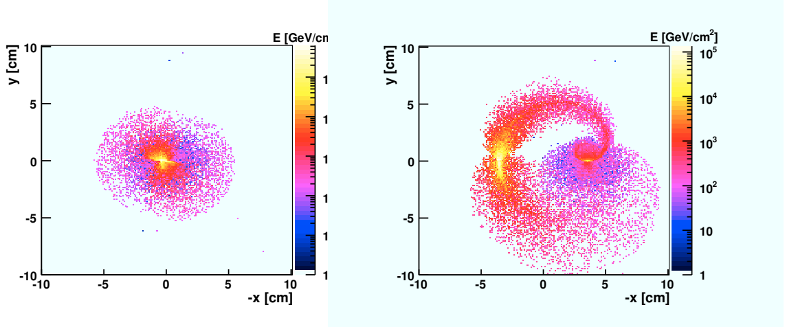
Figure 7.52: Energy distribution in the plane of the BeamCal surface for different magnetic field configurations [75]. Left: The picture actually shows the case of 2 mrad without an additional field, but 14 mrad with an anti-DID are very similar. Most particles reach the hole for the outgoing beam. Right: In the case of 14 mrad with a DID, only high-energy particles reach the hole for the outgoing beam (left spot), whereas low-energy particles are guided into the hole for the incoming beam (right spot). Particles with intermediate energies are swept across the BeamCal surface by the magnetic field.
