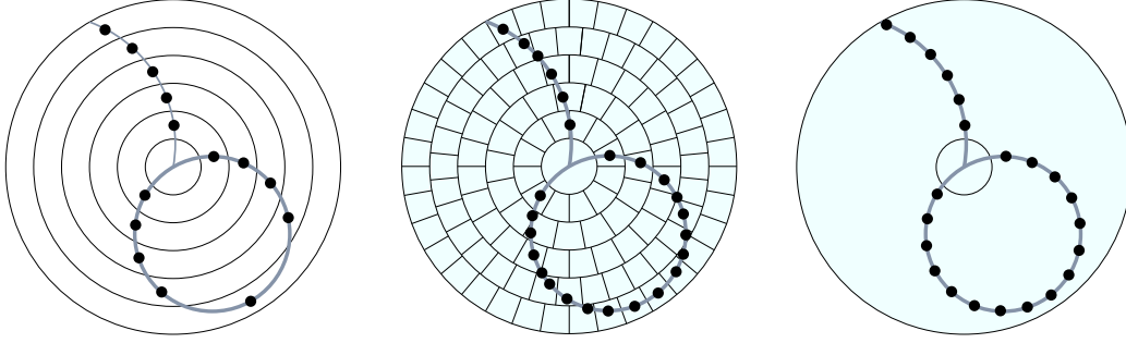
Figure B.2: Possible segmentations of the TPC volume to break simulation steps into smaller pieces. Left: Radial segmentation with artificial gas layers. Middle: Three-dimensional segmentation with artificial voxels. Right: Limitation of the maximum allowed step length, i.e. a segmentation along the line of flight.
