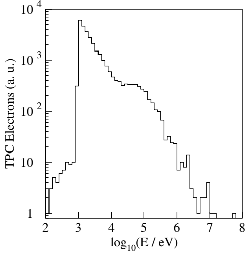
Figure 7.33: Energy distribution of electrons that are created inside the TPC volume
