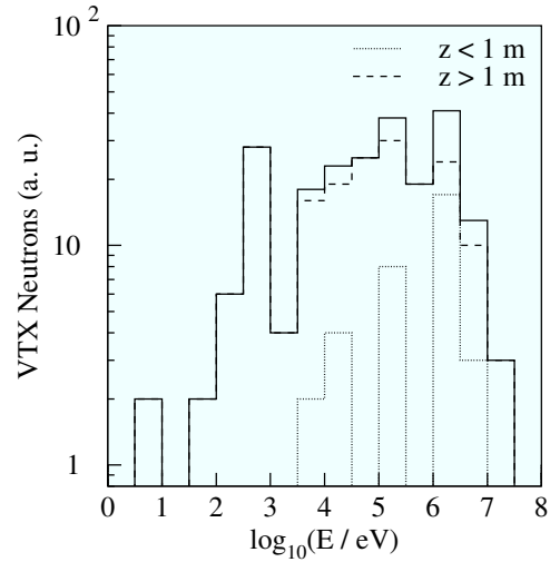
Figure 7.65: Energy distribution of neutrons traversing the vertex detector, using the physics list LHEP_BIC_HP
