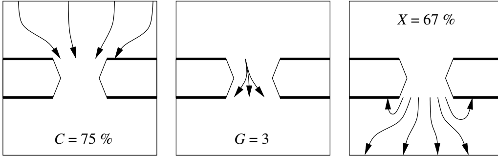
Figure 5.7: Illustration of the collection efficiency (left), the gain (middle), and the extraction efficiency (right) of a GEM. Collection and extraction efficiency are shown for electrons, but corresponding values can also be defined for ions drifting in the opposite direction. The indicated values have merely been chosen for clarification – they are not related to the values in a typical experimental set-up.
