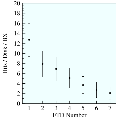
Figure 7.23: Hits on the Forward Tracking Discs of one detector half per bunch crossing, in absolute numbers
