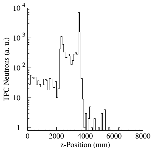
Figure 7.27: Origins of neutrons that enter the TPC volume
