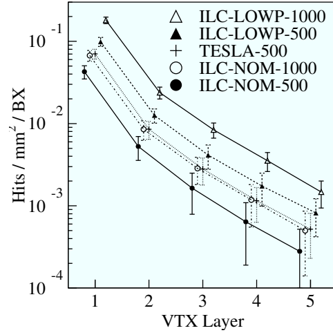
Figure 7.58: Hits on the vertex detector per bunch crossing for different beam parameters, normalised per unit area
