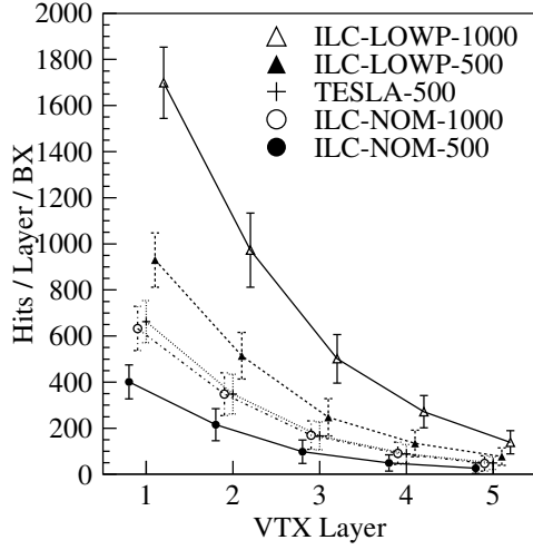
Figure 7.57: Hits on the vertex detector per bunch crossing for different beam parameters, in absolute numbers
