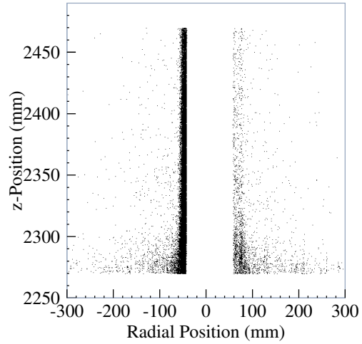
Figure 7.62: Backscattering sources in the LumiCal for an inner radius of 60 mm, top view
