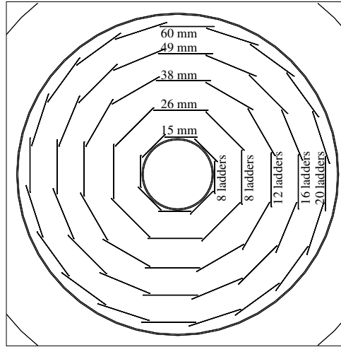
Figure B.1: Geometry of the simulated vertex detector
