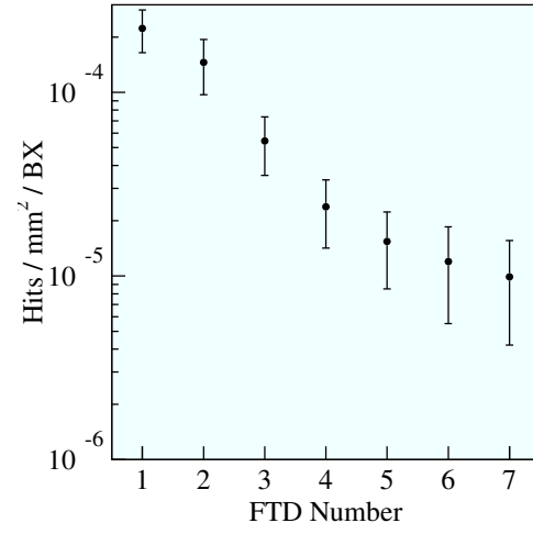
Figure 7.24: Hits on the Forward Tracking Discs per bunch crossing, normalised per unit area
