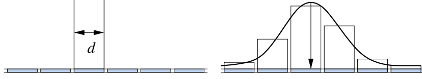
Figure 5.11: If a signal is found only on a single pad, its position cannot be determined with a precision better than d/\sqrt{12} (“hodoscope limit”). In the case of charge sharing between several pads, the position can be reconstructed much more precisely.
