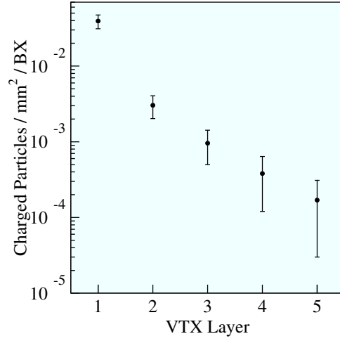
Figure 7.11: Electrons and positrons traversing the vertex detector per bunch crossing, normalised per unit area
