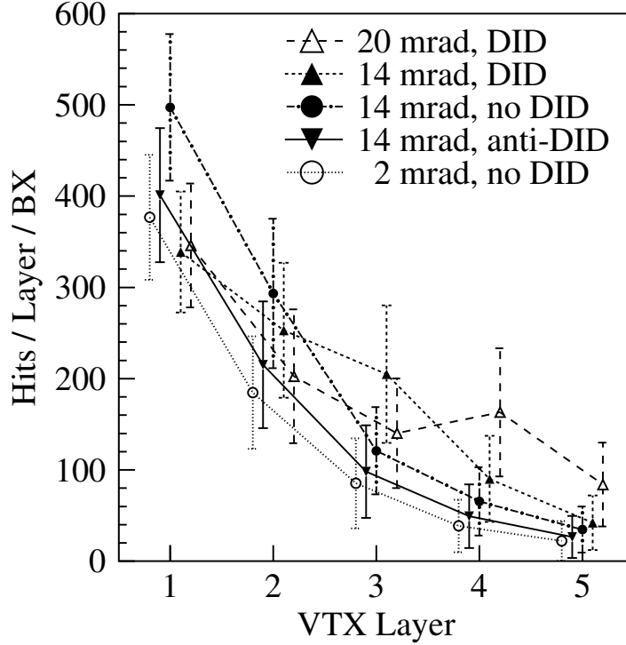
Figure 7.51: Hits on the vertex detector per bunch crossing for different crossing angles and magnetic field configurations
