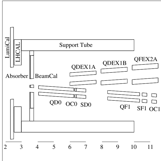
Figure 6.4: Geometry of the simulated forward mask in the xz -plane, compressed by a factor of 10 in z -direction (values are given in metres)
