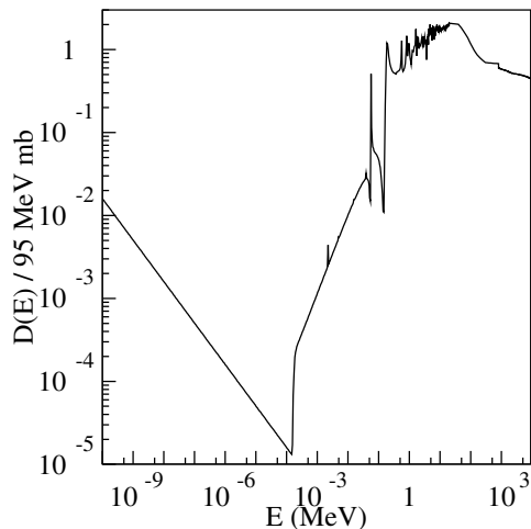
Figure 7.20: Relative neutron-induced displacement damage in silicon in dependency of the incident neutron energy [140]. The plot combines measured data from different sources for 0.1 \text{ meV} < E < 20 \text{ MeV} [141], 20 \text{ MeV} < E < 800 \text{ MeV} [142], and 800 \text{ MeV} < E < 9 \text{ GeV} [143].
