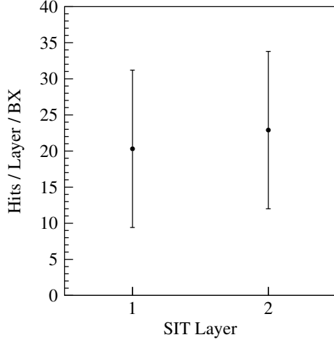
Figure 7.21: Hits on the Silicon Intermediate Tracker per bunch crossing, in absolute numbers
