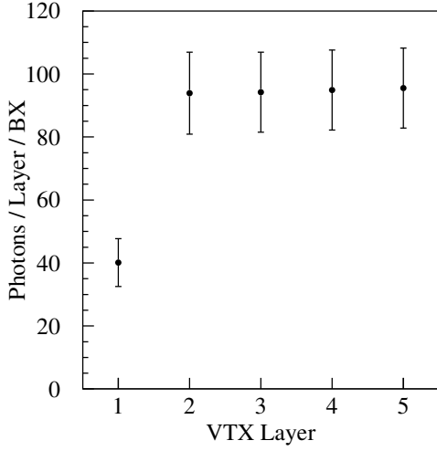
Figure 7.14: Photons traversing the vertex detector per bunch crossing, in absolute numbers
