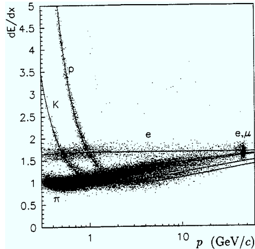
Figure 5.3: Energy loss of pions, kaons, protons, and electrons [84]. The solid lines correspond to the mean energy loss, calculated with the Bethe-Bloch formula. The dots correspond to particles measured in the ALEPH TPC.
