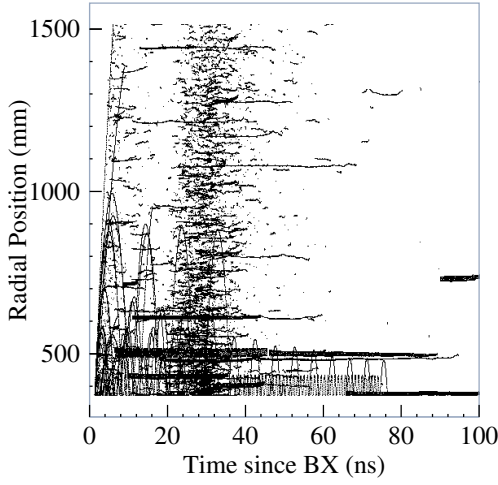
Figure 7.39: Time distribution of hits in the TPC, plotted against the radial position
