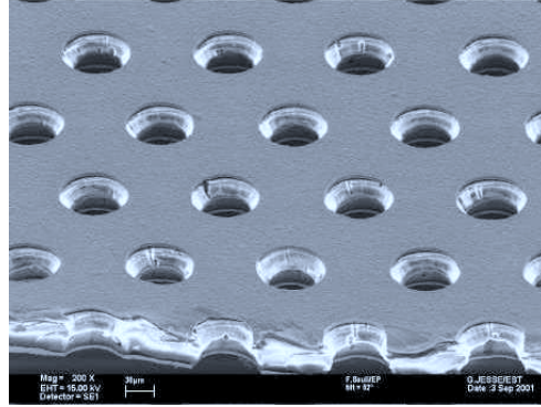
Figure 5.5: The same in reality, imaged with an electron microscope [92]
