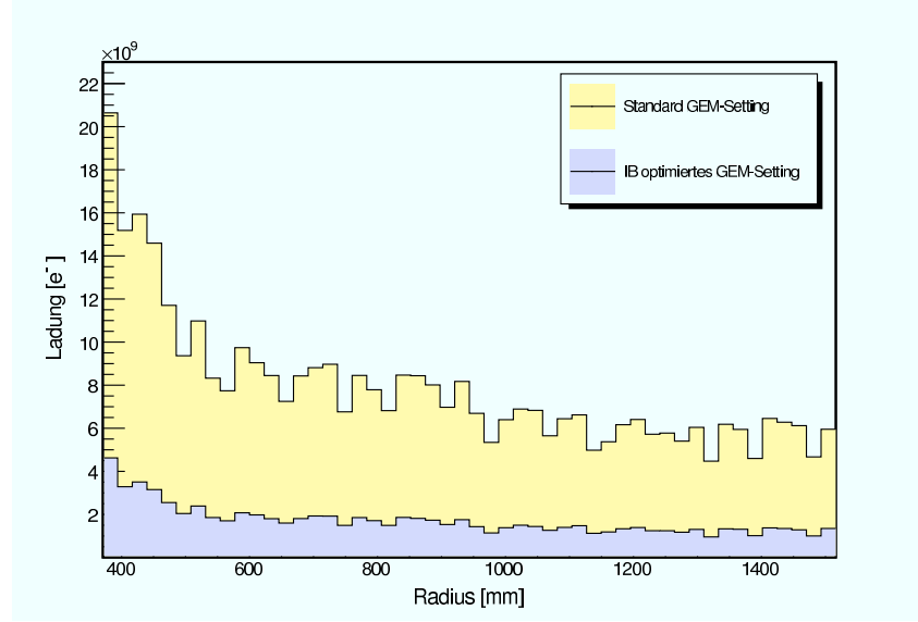
Figure 9.1: Radial charge distribution in a disc of backdrifting ions from a whole bunch train, simulated for standard settings and optimised settings in a triple-GEM structure [161]
