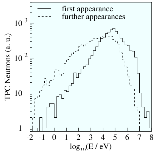
Figure 7.29: Energy distribution of neutrons that enter the TPC volume, at the moment of their entry into the chamber
