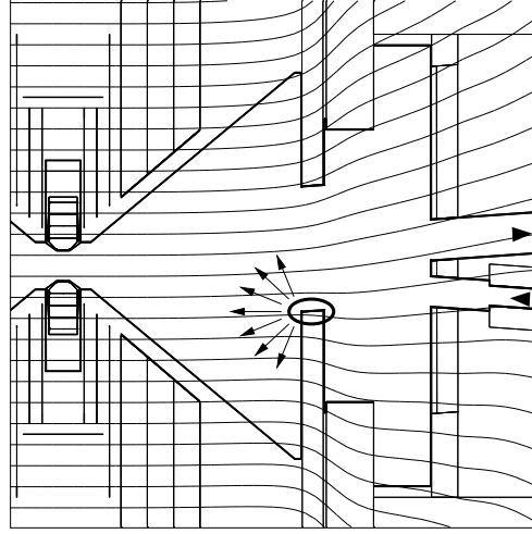
Figure 7.54: Forward region with a decreased inner LumiCal radius of 60 mm. The marked region is a strong source of backscattering photons that can easily reach the TPC.
