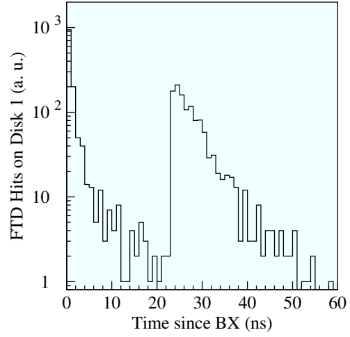
Figure 7.26: Time distribution of hits on the Forward Tracking Discs
