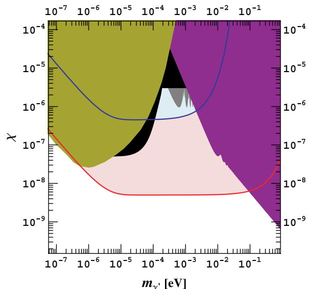
Fig. 1: (Colour on-line) Current bounds on hidden-sector photons from Coulomb law tests [6,7] (green), CAST solar \gamma' searches (purple) [8–11], light-shining-through-walls (LSW) experiments (grey) [12–14] (taken from [15,16]) and distortions of the CMB [17–20]. The blue (red) line shows the sensitivity of the proposed experiment in a conservative (optimistic) scenario. See the text for details.
