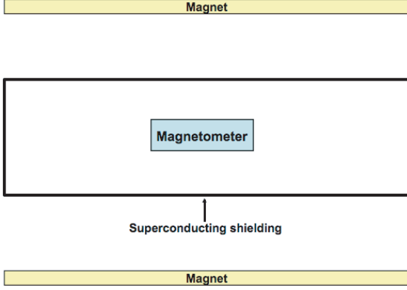
Fig. 2: (Colour on-line) Illustration of the principle of the experiment proposed in this paper. Ordinary magnetic fields are shielded by the superconductor. However, if a hidden U(1) field mixes with the ordinary electromagnetic field some of the magnetic field can convert into a hidden magnetic field, pass through the superconductor and reconvert into an ordinary magnetic field inside the shielding. This field can then be measured by a highly sensitive magnetometer.
