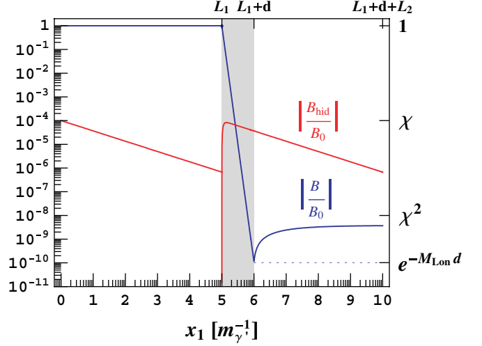
Fig. 3: (Colour on-line) Dependence of the magnetic field \mathbf{B} (blue) and hidden magnetic field \mathbf{B}_{\text{hid}} (red) as a function of the distance from the source ( x_1 ) in our 1-dimensional setup. Both quantities are normalized to the value \mathbf{B}_0 . The dotted line represents the evolution of \mathbf{B} in the absence of the hidden field ( \chi \rightarrow 0 ). Near the external (left) surface of the superconducting shield \mathbf{B}_{\text{hid}} changes sign from negative to positive, hence the abrupt fall to zero. For better visibility we have chosen not too extreme values: \chi = 10^{-4} , m_{\gamma'} L_1 = m_{\gamma'} L_2 = 5 , m_{\gamma'} d = 1 and 23 m_{\gamma'} = M_{\text{Lon}} . For m_{\gamma'} d \ll 1 \ll L_{1,2} m_{\gamma'} the evolution approaches \chi^2 , but for the chosen parameters the result is a bit smaller because the hidden field is a bit damped inside the shielding due to m_{\gamma'} d = 1 .
