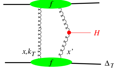
Figure 1: A simple graph for central exclusive Higgs production. The blobs represent the generalised gluon distribution.
