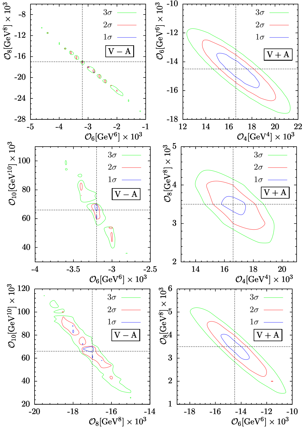
Figure 4: 3-parameter fits in the V - A and V + A channels: 1-, 2- and 3\sigma confidence regions defined by contours of constant \chi^2_L in the plane of two of the fitted parameters and located at the central value of the third one. The central values (see Tab. 2) are marked by dashed lines.
