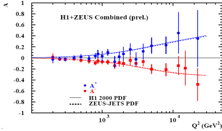
Figure 2. Measurements of the polarisation asymmetries A^\pm based on preliminary combined H1 and ZEUS cross sections. The error bars denote the total uncertainty which is dominated by the uncorrelated error contributions. The curves describe the theoretical predictions in NLO QCD as obtained in fits to the H1 inclusive data and to the inclusive and jet ZEUS data, respectively. Both fits have been performed using the unpolarised HERA I data.
