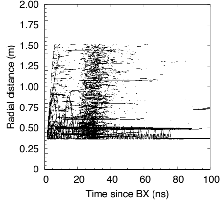
Figure 7: Radius-vs-time distribution of hits in the TPC
