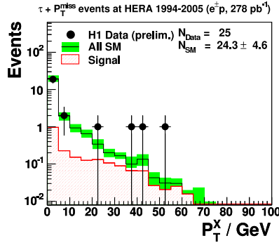
Figure 9. The hadronic transverse momentum distribution of \tau + P_T^{\text{miss}} events observed by the H1 experiment is compared to the SM expectation.
