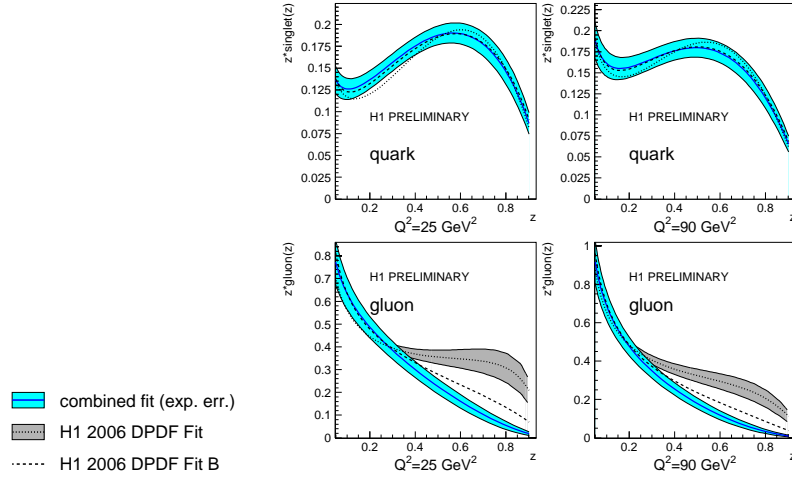
Figure 4. The diffractive singlet density (top) and diffractive gluon density (bottom) for two values of the hard scale \mu: 25 \text{ GeV}^2 (left) and 90 \text{ GeV}^2 (right). The blue line indicates the combined fit, surrounded by the experimental uncertainty band in light blue. For comparison, the two dashed lines show two fit results from the inclusive cross sections alone.
