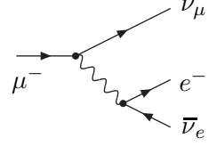
Figure 5.7: \mu decay
