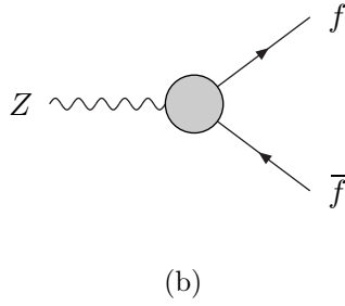
Figure 5.2: Decays of the W and Z bosons into two fermions. In W decays, the fermion and antifermion can have different flavour. The grey blobs indicate higher order corrections which must be included to match the experimental precision.
