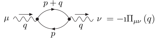
(b) The vacuum polarisation
