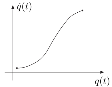
Figure 2.1: Particle moving in one dimension
