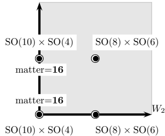
FIG. 2: Local gauge symmetries in the \text{SO}(4) plane (at the origin in the G_2 and \text{SU}(3) planes). Two \mathbf{16} -plets arise from the orbifold fixed points.
