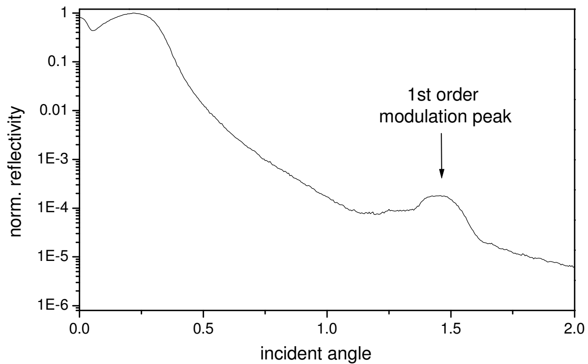
Figure 1: XRR curve of the sample CTS-11. The maximum is due to the modulated nature of the multilayer and the angular position corresponds to the repeating tri-layer thickness.
