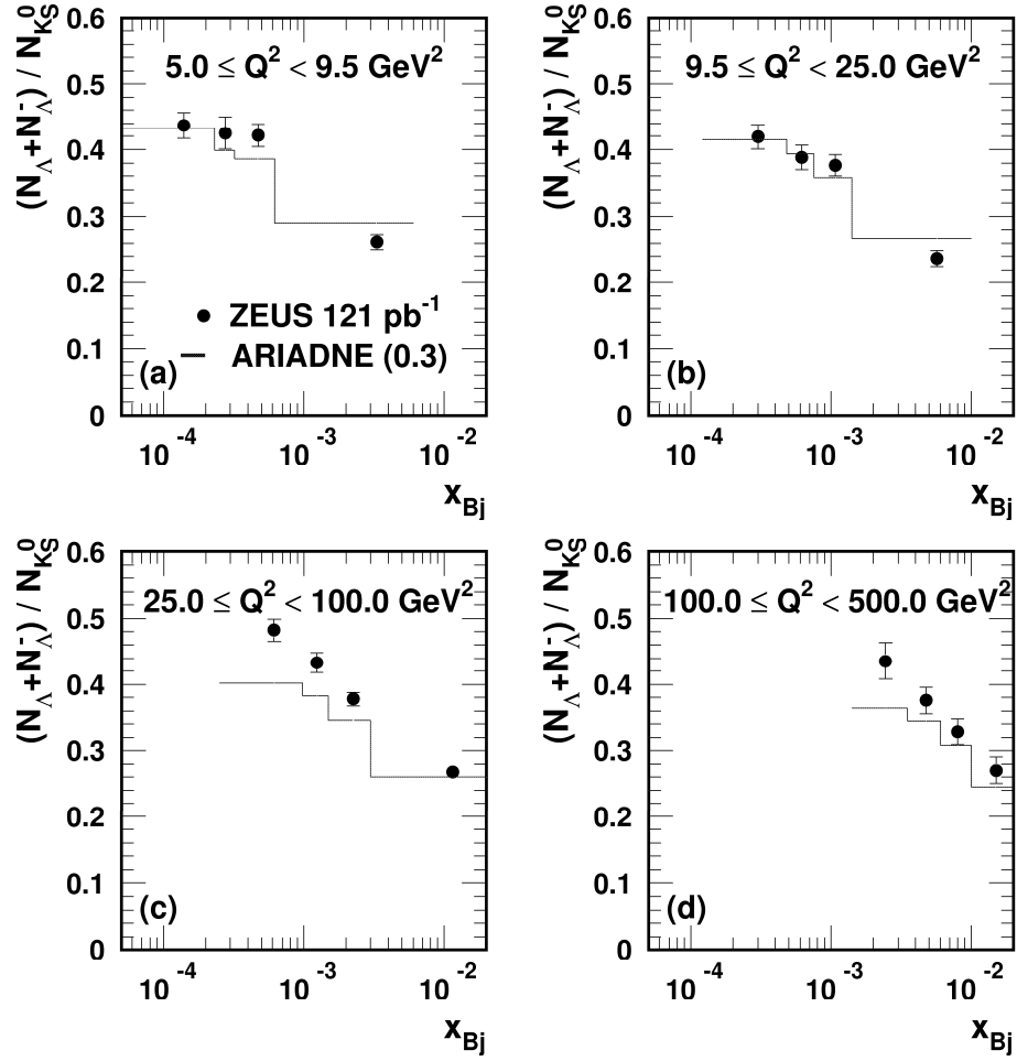
Figure 14: The ratio \frac{N(\Lambda) + N(\bar{\Lambda})}{N(K_S^0)} as a function of x_{Bj} for four bins of Q^2 , in the range 0.6 < P_T^{\text{LAB}} < 2.5 \text{ GeV} and |\eta^{\text{LAB}}| < 1.2 for events with Q^2 > 5 \text{ GeV}^2 and 0.02 < y < 0.95 . Statistical errors only are shown. The histograms show predictions from ARIADNE with a strangeness-suppression factor of 0.3.
