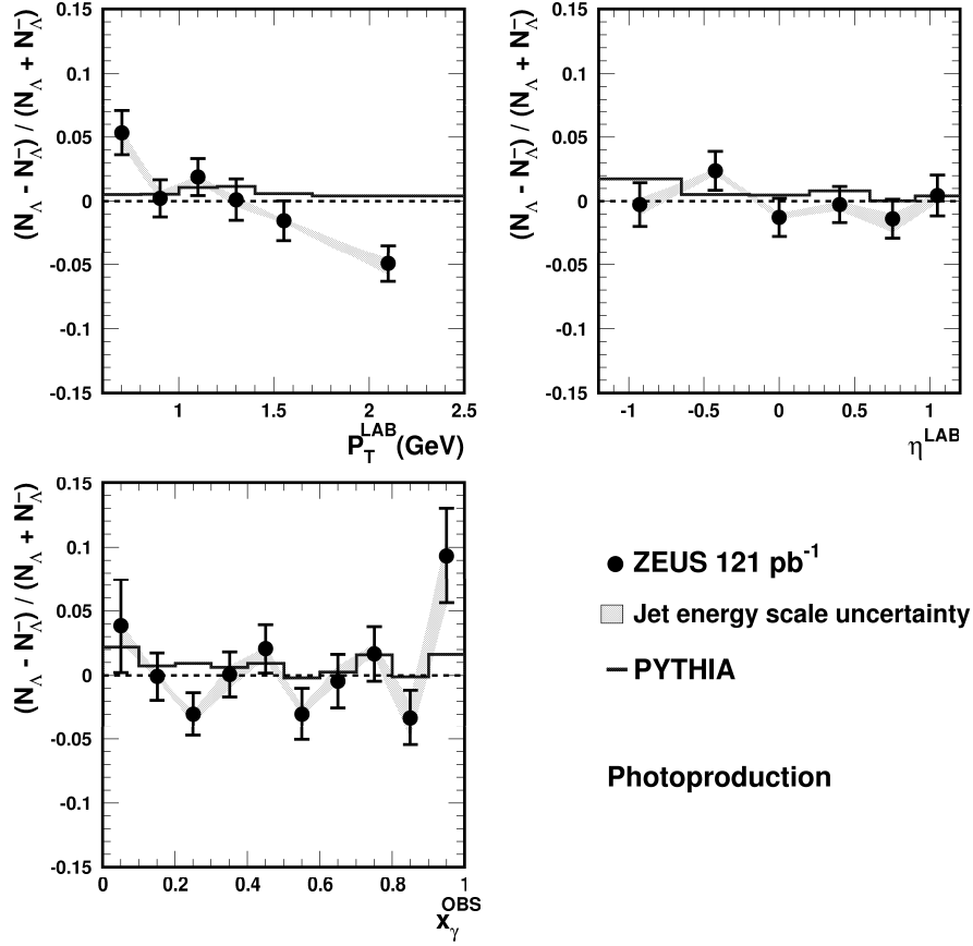
Figure 10: The ratio \frac{N(\Lambda) - N(\bar{\Lambda})}{N(\Lambda) + N(\bar{\Lambda})} as a function of P_T^{\text{LAB}} , \eta^{\text{LAB}} and x_{\gamma}^{\text{OBS}} , in the range 0.6 < P_T^{\text{LAB}} < 2.5 \text{ GeV} and |\eta^{\text{LAB}}| < 1.2 for events with Q^2 < 1 \text{ GeV}^2 , 0.2 < y < 0.85 and at least two jets both satisfying E_T^{\text{jet}} > 5 \text{ GeV} and |\eta^{\text{jet}}| < 2.4 . Statistical errors are shown, together with the uncertainty arising from the jet energy scale (shaded band). The solid histogram shows the prediction from PYTHIA (with multiple interactions).
