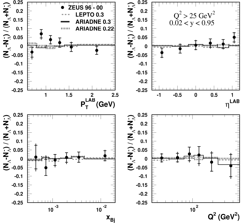
Figure 9: The ratio \frac{N(\Lambda) - N(\bar{\Lambda})}{N(\Lambda) + N(\bar{\Lambda})} as a function of P_T^{\text{LAB}} , \eta^{\text{LAB}} , x_{\text{Bj}} and Q^2 , in the range 0.6 < P_T^{\text{LAB}} < 2.5 \text{ GeV} and |\eta^{\text{LAB}}| < 1.2 for events with Q^2 > 25 \text{ GeV}^2 and 0.02 < y < 0.95 . Statistical errors (inner error bars) and the systematic uncertainties added in quadrature are shown. The solid histogram shows the prediction from ARIADNE with a strangeness-suppression factor of 0.3. The dotted line shows the prediction of ARIADNE with a strangeness-suppression factor of 0.22. The dashed line shows the prediction of LEPTO, with a strangeness-suppression factor of 0.3.
