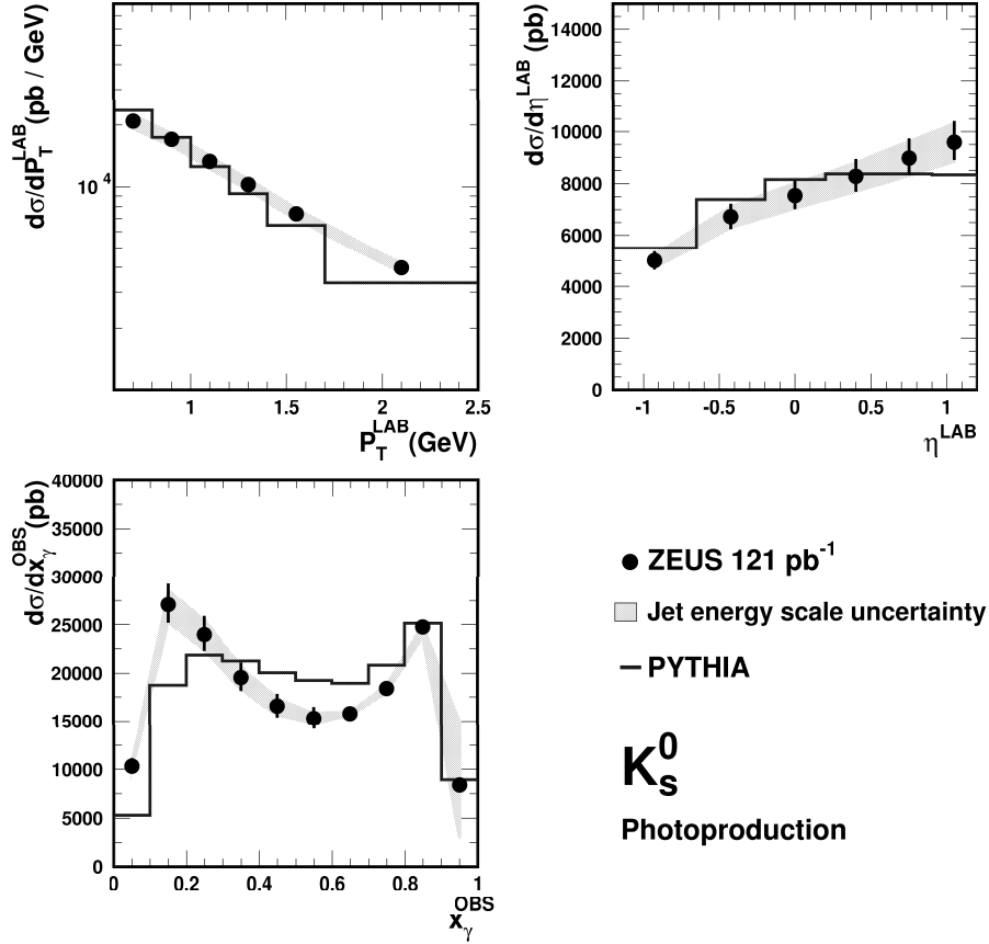
Figure 7: Differential K_S^0 cross sections as a function of P_T^{\text{LAB}} , \eta^{\text{LAB}} and x_\gamma^{\text{OBS}} , in the range 0.6 < P_T^{\text{LAB}} < 2.5 \text{ GeV} and |\eta^{\text{LAB}}| < 1.2 for events with Q^2 < 1 \text{ GeV}^2 , 0.2 < y < 0.85 and at least two jets both satisfying E_T^{\text{jet}} > 5 \text{ GeV} and |\eta^{\text{jet}}| < 2.4 . Statistical errors are shown, unless smaller than the point size, together with the systematic uncertainty arising from the trigger efficiency added in quadrature. The uncertainty arising from the jet energy scale is also shown (shaded band). The solid histogram shows the prediction from PYTHIA (with multiple interactions), normalised to the data.
