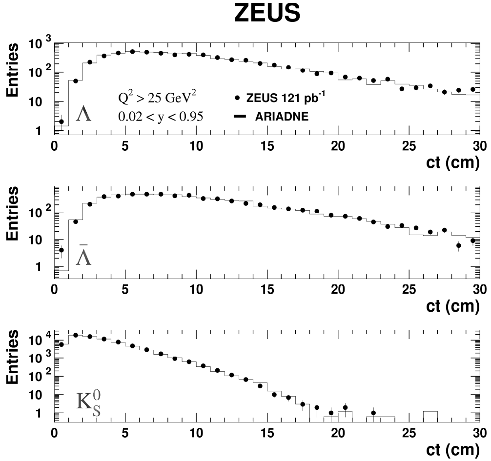
Figure 2: Detector-level distributions of ct , where t is the reconstructed lifetime, for \Lambda , \bar{\Lambda} and K_S^0 samples for data and ARIADNE. The ARIADNE histogram is normalised to the same number of events as the data. Statistical errors are shown unless smaller than the point size.
