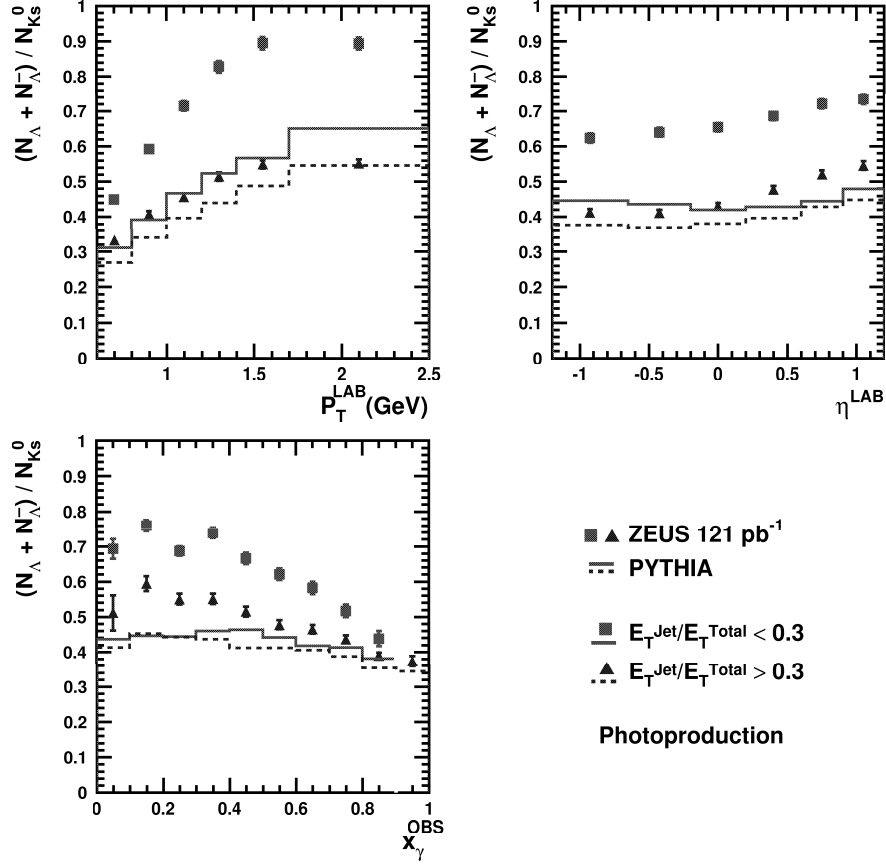
Figure 17: The ratio \frac{N(\Lambda) + N(\bar{\Lambda})}{N(K_s^0)} as a function of P_T^{\text{LAB}} , \eta^{\text{LAB}} and x_{\gamma}^{\text{OBS}} , in the range 0.6 < P_T^{\text{LAB}} < 2.5 \text{ GeV} and |\eta^{\text{LAB}}| < 1.2 for events with Q^2 < 1 \text{ GeV}^2 , 0.2 < y < 0.85 and at least two jets both satisfying E_T^{\text{jet}} > 5 \text{ GeV} and |\eta^{\text{jet}}| < 2.4 . The ratios from the fireball-enriched sample (squares) and the fireball-depleted sample (triangles) are shown for the data. The prediction from PYTHIA for the fireball-enriched (solid line) and for the fireball-depleted (dashed line) samples are shown. Statistical errors are shown. The highest x_{\gamma}^{\text{OBS}} bin ( 0.9 < x_{\gamma}^{\text{OBS}} < 1.0 ) of the fireball enriched sample is omitted due to insufficient statistics.
