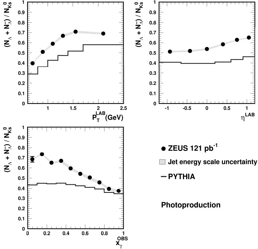
Figure 15: The ratio \frac{N(\Lambda) + N(\bar{\Lambda})}{N(K_S^0)} as a function of P_T^{\text{LAB}} , \eta^{\text{LAB}} and x_\gamma^{\text{OBS}} , in the range 0.6 < P_T^{\text{LAB}} < 2.5 \text{ GeV} and |\eta^{\text{LAB}}| < 1.2 for events with Q^2 < 1 \text{ GeV}^2 , 0.2 < y < 0.85 and at least two jets both satisfying E_T^{\text{jet}} > 5 \text{ GeV} and |\eta^{\text{jet}}| < 2.4 . The statistical errors are shown, unless smaller than the point size. The shaded band shows the uncertainty arising from the jet energy scale. The solid histogram shows the prediction from PYTHIA (with multiple interactions).
