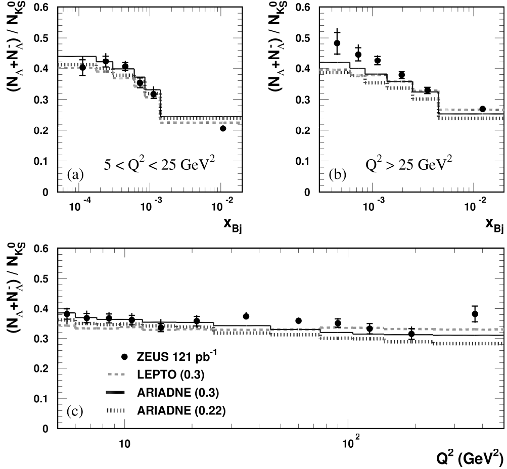
Figure 12: The ratio \frac{N(\Lambda) + N(\bar{\Lambda})}{N(K_S^0)} as a function of x_{Bj} and Q^2 in the range 0.6 < P_T^{\text{LAB}} < 2.5 \text{ GeV} and |\eta^{\text{LAB}}| < 1.2 for events with a) 5 < Q^2 < 25 \text{ GeV}^2 , 0.02 < y < 0.95 b) Q^2 > 25 \text{ GeV}^2 , 0.02 < y < 0.95 and c) Q^2 > 5 \text{ GeV}^2 , 0.02 < y < 0.95 . Statistical errors (inner error bars) and the systematic uncertainties added in quadrature are shown. The solid histogram shows the prediction from ARIADNE with a strangeness-suppression factor of 0.3. The dotted line shows the prediction of ARIADNE with a strangeness-suppression factor of 0.22. The dashed line shows the prediction of LEPTO, with a strangeness-suppression factor of 0.3.
