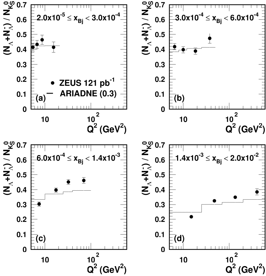
Figure 13: The ratio \frac{N(\Lambda) + N(\bar{\Lambda})}{N(K_S^0)} as a function of Q^2 for four bins of x_{Bj} , in the range 0.6 < P_T^{\text{LAB}} < 2.5 \text{ GeV} and |\eta^{\text{LAB}}| < 1.2 for events with Q^2 > 5 \text{ GeV}^2 and 0.02 < y < 0.95 . Statistical errors only are shown. The histograms show predictions from ARIADNE with a strangeness-suppression factor of 0.3.
