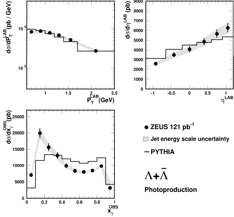
Figure 8: Differential \Lambda + \bar{\Lambda} cross sections as a function of P_T^{\text{LAB}} , \eta^{\text{LAB}} and x_\gamma^{\text{OBS}} , in the range 0.6 < P_T^{\text{LAB}} < 2.5 GeV and |\eta^{\text{LAB}}| < 1.2 for events with Q^2 < 1 GeV 2 , 0.2 < y < 0.85 and at least two jets both satisfying E_T^{\text{jet}} > 5 GeV and |\eta^{\text{jet}}| < 2.4 . Statistical errors are shown, unless smaller than the point size, together with the systematic uncertainty arising from the trigger efficiency added in quadrature. The uncertainty arising from the jet energy scale is also shown (shaded band). The solid histogram shows the prediction from PYTHIA (with multiple interactions), normalised to the data.
