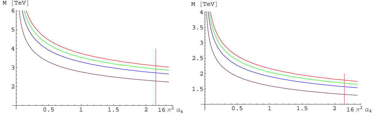
Figure 16: Dependence of the resonance mass for the vector triplet on \alpha_4 in the special isospin-violating case g_\rho = -h_\rho for different assumed width to mass ratios (in red f_\rho = \Gamma_\rho/M_{\rho^+} = 1.0 , blue 0.8, green 0.6, brown 0.3, respectively). On the left is the charged resonance, on the right the neutral one.
