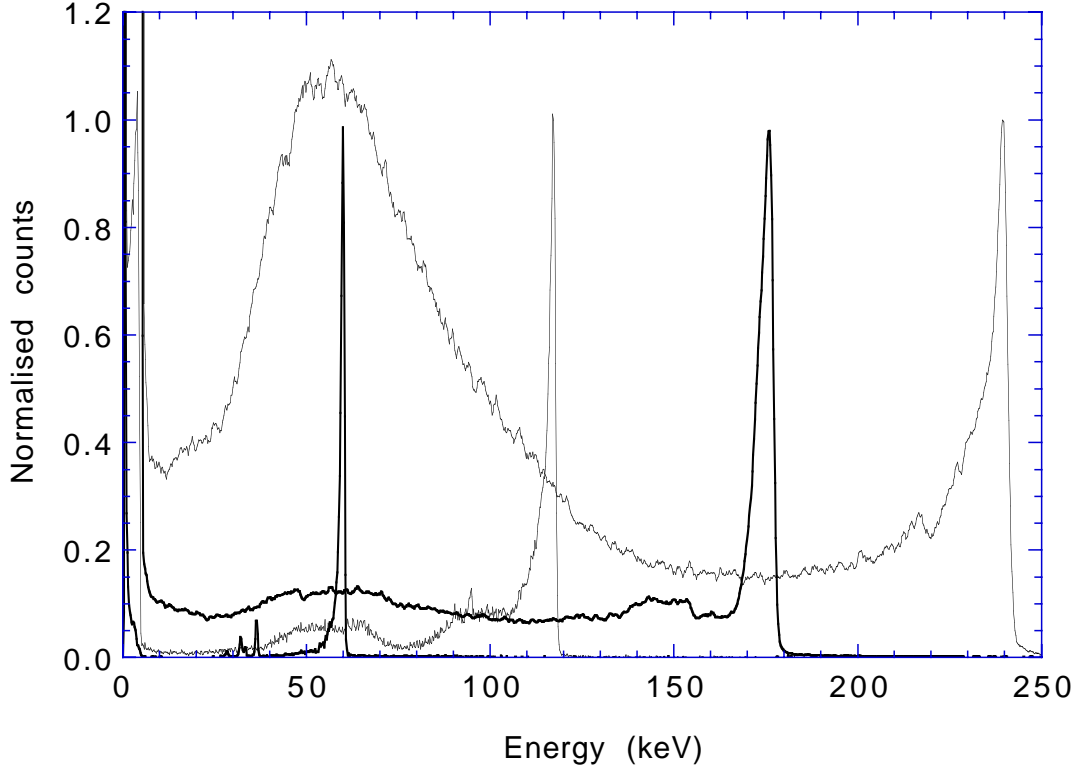
Fig. 3. Composite pulse height spectra of monoenergetic lines measured at the ESRF. The beam size was 20 \times 20 \mu\text{m}^2 , incident at the center of the detector.
