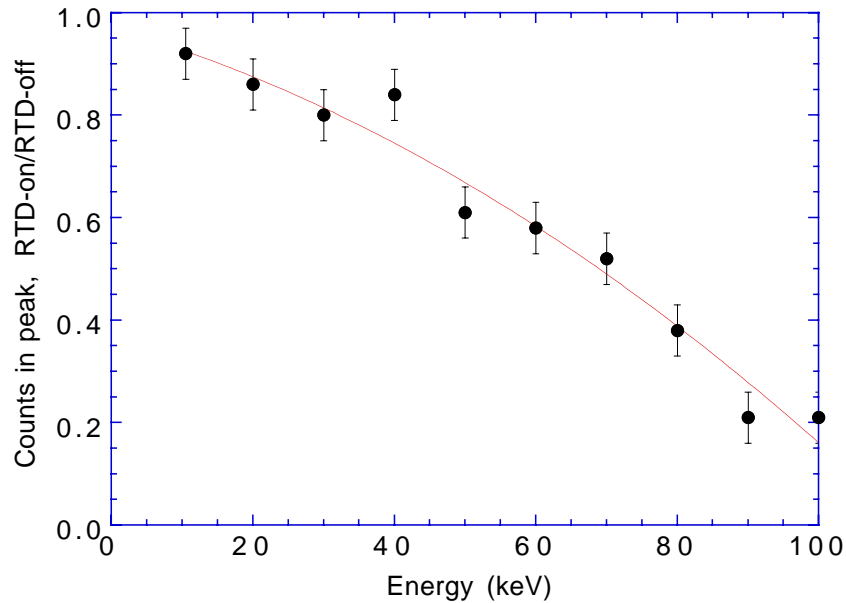
Fig. 7. The ratio of the counts in the photopeak, measured with and without the rise time discrimination (RTD) illustrating the loss of relative efficiency when RTD is employed.
