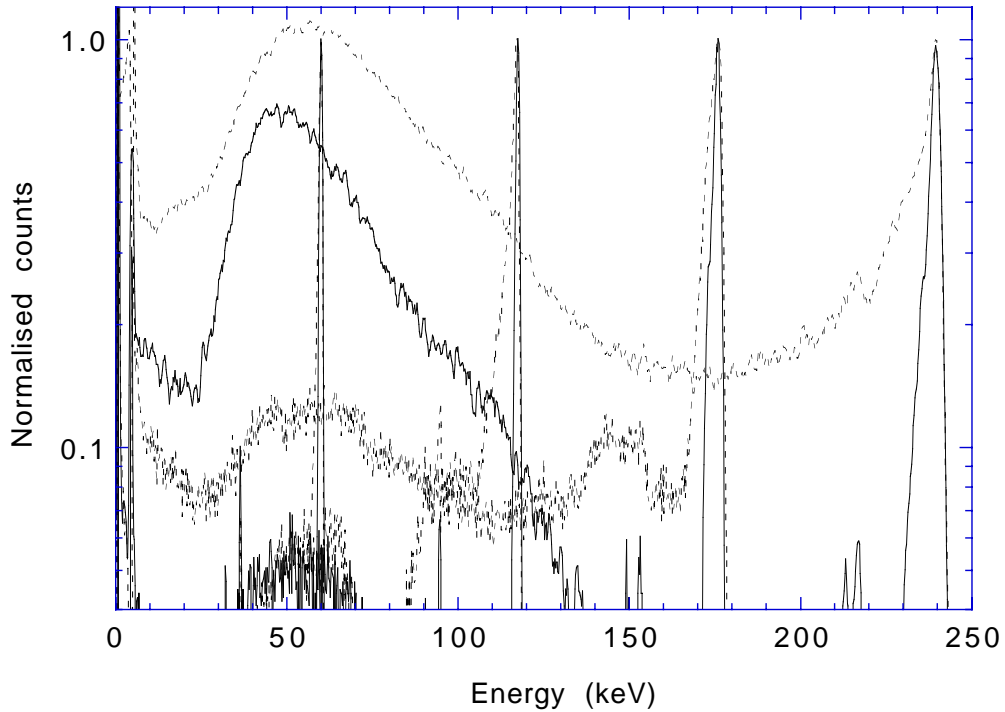
Fig. 6. A composite of energy spectra measured at the ESRF using pencil beam illumination with risetime discrimination switched-in (solid curves) and switched-out (dotted curves).
