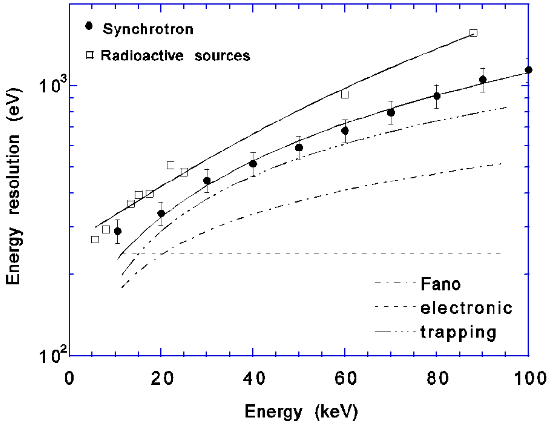
Fig. 4. The energy resolution \Delta E measured using a 20 \times 20 \mu\text{m}^2 pencil beam illumination. The solid line shows the best-fit resolution function to the data. The individual components to the FWHM are also shown for this curve. These are: the noise due to carrier generation, or Fano noise, \Delta E_F , electronic noise due to leakage current and amplifier shot noise, \Delta E_e , and incomplete charge collection or trapping noise, \Delta E_c . For completeness, we also show the measured FWHM energy resolution using full-area illumination with radioactive sources.
