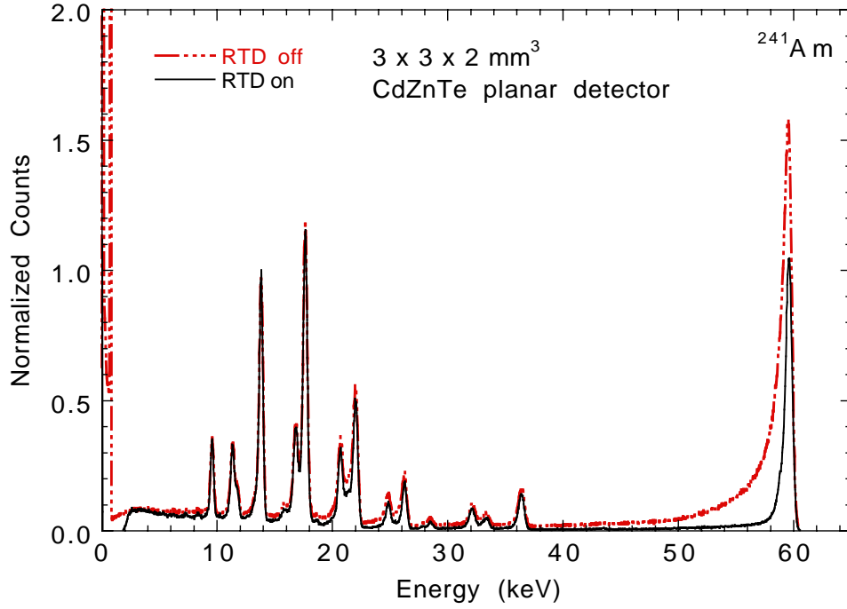
Fig. 5. Two ^{241}\text{Am} spectra taken with a 3 \times 3 \times 2 \text{ mm}^3 CdZnTe detector, illustrating the effectiveness of rise-time discrimination. From the figure, we see that the hole tailing is substantially reduced when RTD is used and in fact the FWHM energy resolution improves from \sim 1 \text{ keV} to 700 \text{ eV} at 59.54 \text{ keV} . However, an energy dependent decrease in photopeak efficiency is also apparent.
