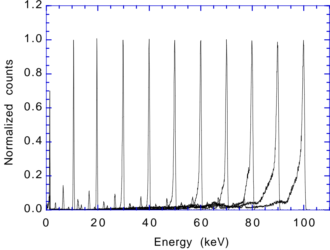
Fig. 2. Composite pulse height spectra of monoenergetic lines measured at HASYLAB. The beam size was 20 \times 20 \mu\text{m}^2 , incident at the center of the detector.
