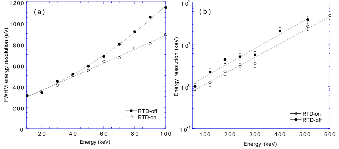
Fig. 8. The measured FWHM energy resolution as function of energy with the RTD switched on and switched off. (a) low energies measured at HASYLAB and, (b) high energies measured at the ESRF.
