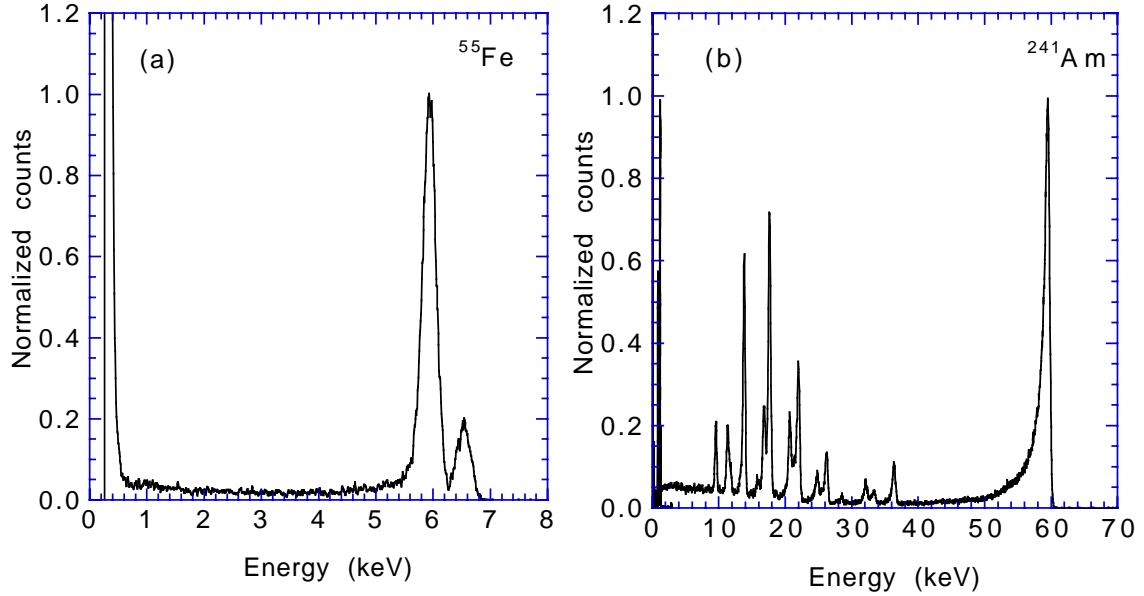
Fig. 1. The measured response of a 3 \times 3 \times 2 \text{ mm}^3 thick CdZnTe detector to a) ^{55}\text{Fe} and b) ^{241}\text{Am} under full-area illumination.
